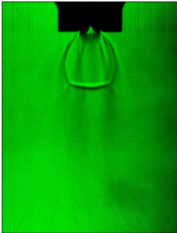
Figure 59. Shadowgraph image, X_{\text{CH}_4} = 0.1 , nozzle #7, d = 0.5\text{mm} , T_r = 1.04 , P_r = 1.03
