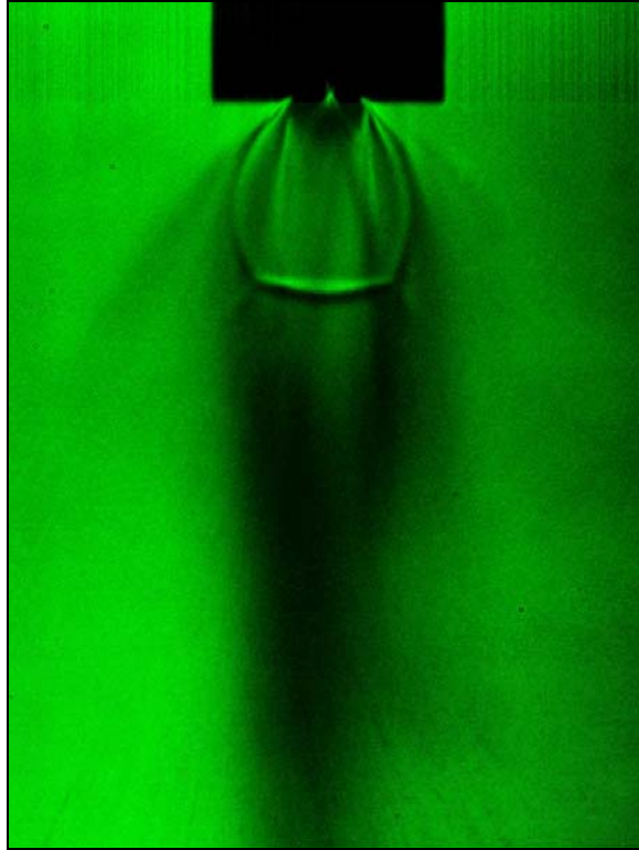
Figure 52. Shadowgraph image, X_{\text{CH}_4} = 0.1 , nozzle #6, d = 0.5\text{mm} , T_r = 1.00 , P_r = 1.04
