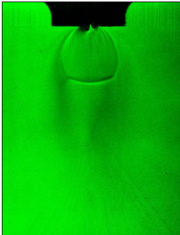
Figure 32. Shadowgraph image, ethylene, nozzle #1, d = 0.5\text{mm} , T_r = 1.01 , P_r = 1.03
