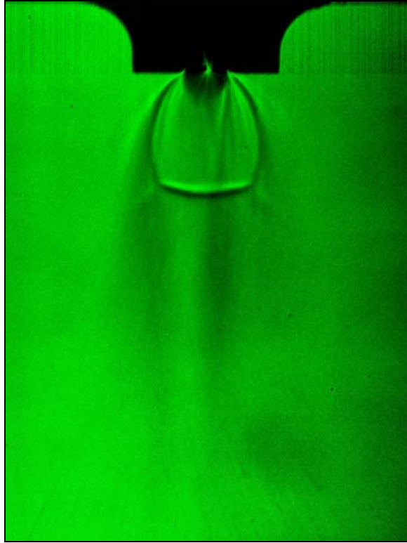
Figure 50. Shadowgraph image, X_{\text{CH}_4} = 0.1 , nozzle #1, d = 0.5\text{mm} , T_r = 1.02 , P_r = 1.04
