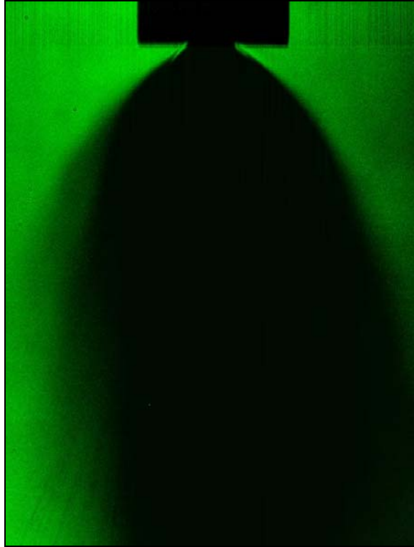
Figure 60. Shadowgraph image, X_{\text{CH}_4} = 0.1 , nozzle #9, d = 0.5\text{mm} , T_r = 1.00 , P_r = 1.04
