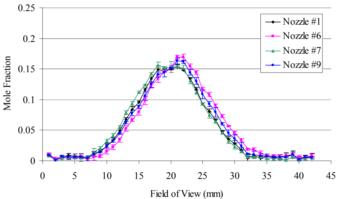
Figure 93. Ethylene mole fraction, X_{CH_4}=0.1 mixture, T_r = 1.04 , without accumulated number density.
