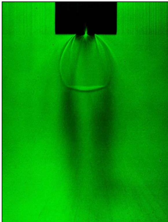
Figure 61. Shadowgraph image, X_{\text{CH}_4} = 0.1 , nozzle #9, d = 0.5\text{mm} , T_r = 1.01 , P_r = 1.01
