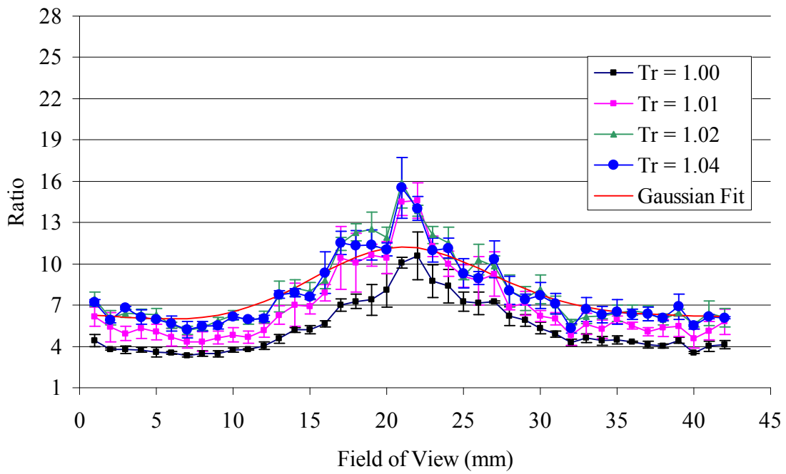
Figure 107. Mole fraction ratio, X_{CH_4}=0.1 mixture, nozzle #9.
