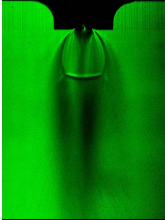
Figure 48. Shadowgraph image, X_{\text{CH}_4} = 0.1 , nozzle #1, d = 0.5\text{mm} , T_r = 1.00 , P_r = 1.04
