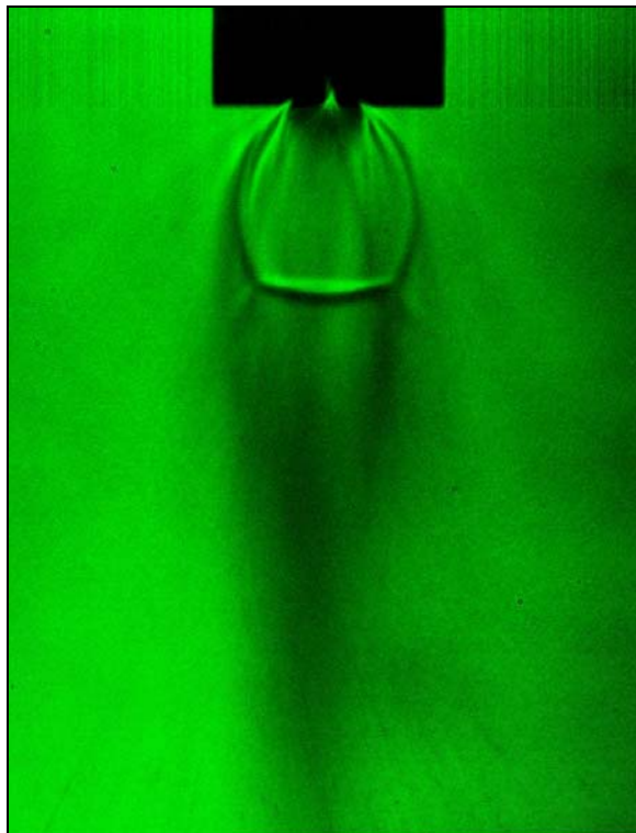
Figure 53. Shadowgraph image, X_{\text{CH}_4} = 0.1 , nozzle #6, d = 0.5\text{mm} , T_r = 1.01 , P_r = 1.04
