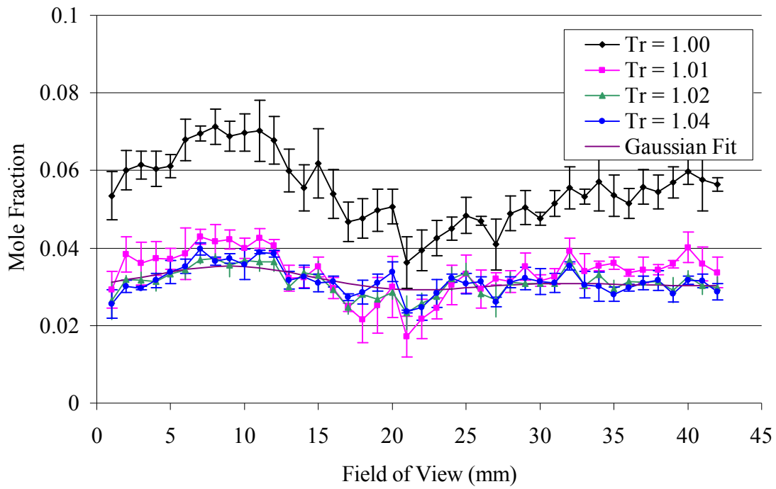
Figure 98. Methane mole fraction, X_{CH_4} = 0.1 mixture, nozzle #7.
