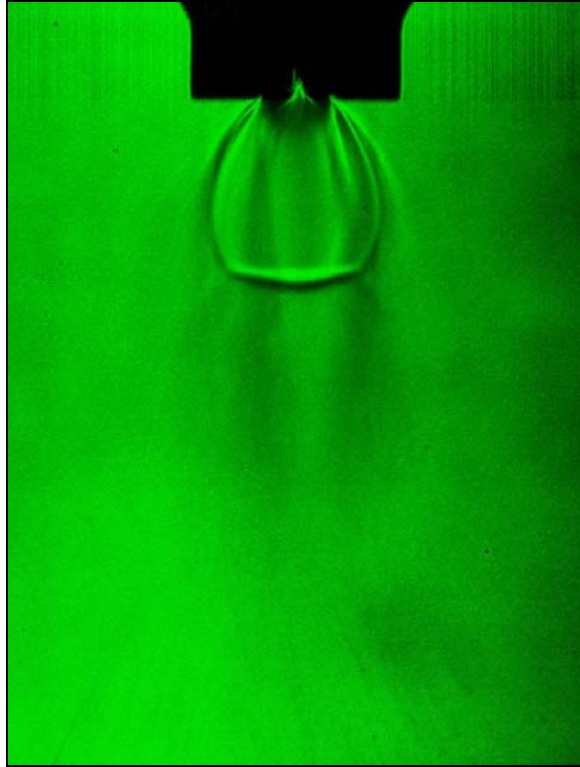
Figure 58. Shadowgraph image, X_{\text{CH}_4} = 0.1 , nozzle #7, d = 0.5\text{mm} , T_r = 1.03 , P_r = 1.04
