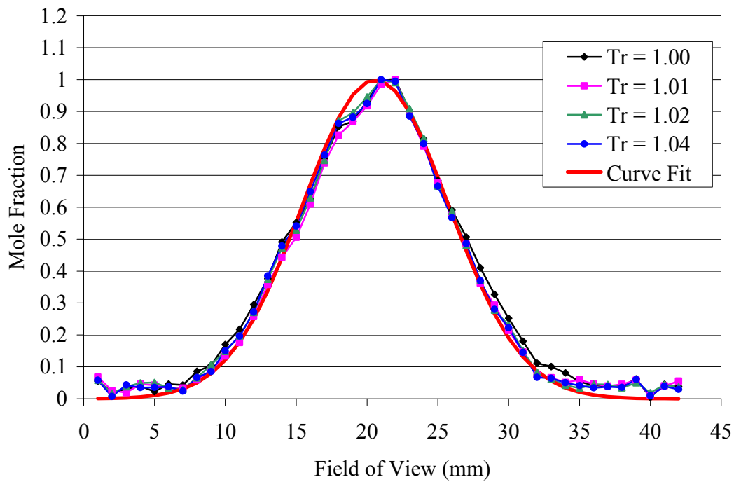
Figure 89. Normalized ethylene mole fraction, X_{CH_4} = 0.1 mixture, nozzle #9.
