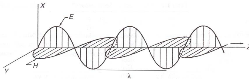
Figure 8. Electromagnetic radiation [16].
