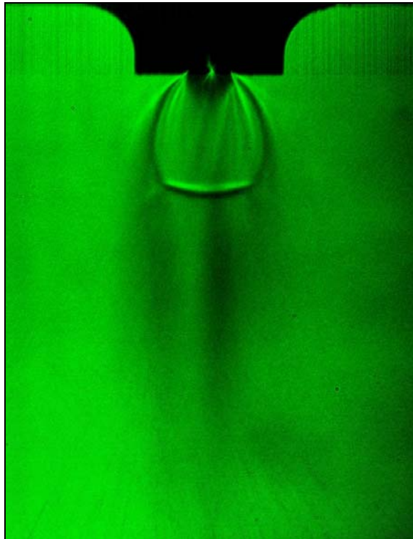
Figure 49. Shadowgraph image, X_{\text{CH}_4} = 0.1 , nozzle #1, d = 0.5\text{mm} , T_r = 1.01 , P_r = 1.04
