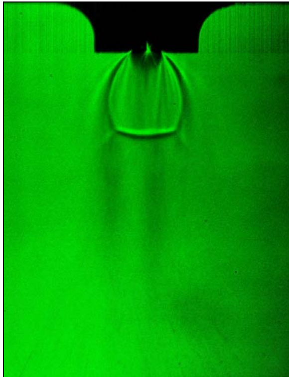
Figure 51. Shadowgraph image, X_{\text{CH}_4} = 0.1 , nozzle #1, d = 0.5\text{mm} , T_r = 1.04 , P_r = 1.04
