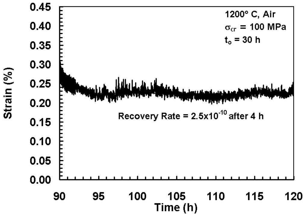
Figure 30. Strain vs. time curve for N720/A composite obtained during recovery period of cycle 2 in cyclic creep test with \sigma_{\max} = 100 MPa and t_0 = 30 h conducted at 1200 °C in laboratory air. Recovery saturation after \sim 4 h at near zero stress is evident.
