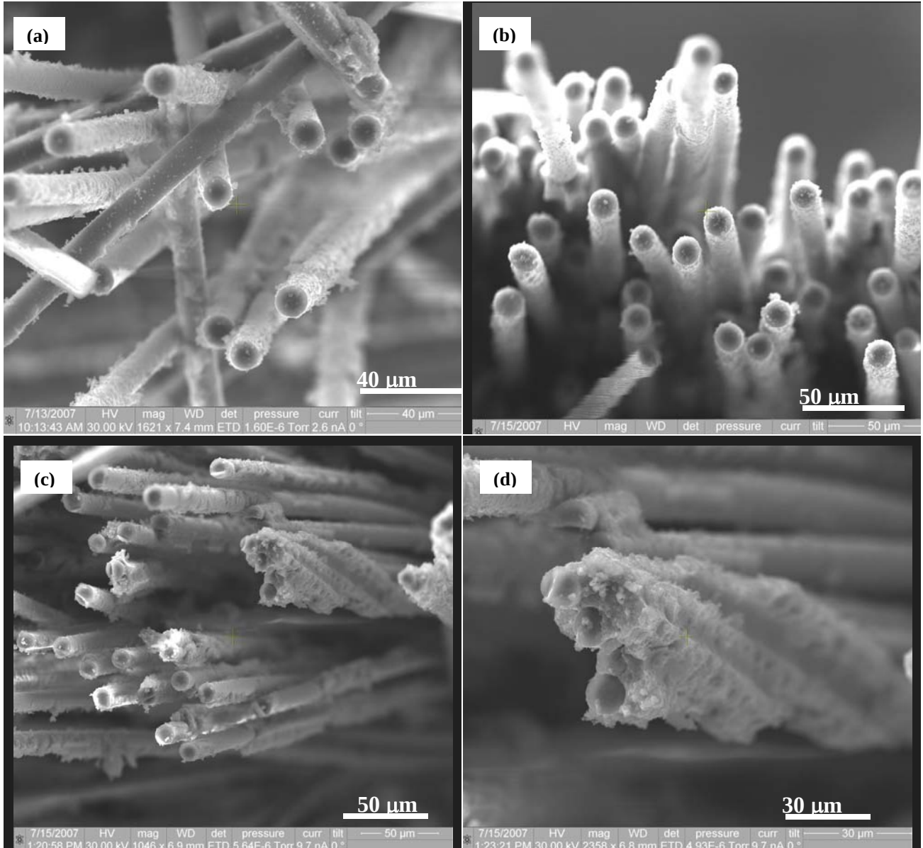
Figure 51. Fracture surfaces of the N720/A specimens subjected to cyclic creep and recovery tests at 1200 °C in laboratory air: (a) \sigma_{\text{max}} = 100 MPa and t_0 = 1 h, (b) \sigma_{\text{max}} = 100 MPa and t_0 = 30 h, and (c-d) \sigma_{\text{max}} = 125 MPa and t_0 = 1 h. All micrographs show matrix particles bonded to the pulled out fibers.
