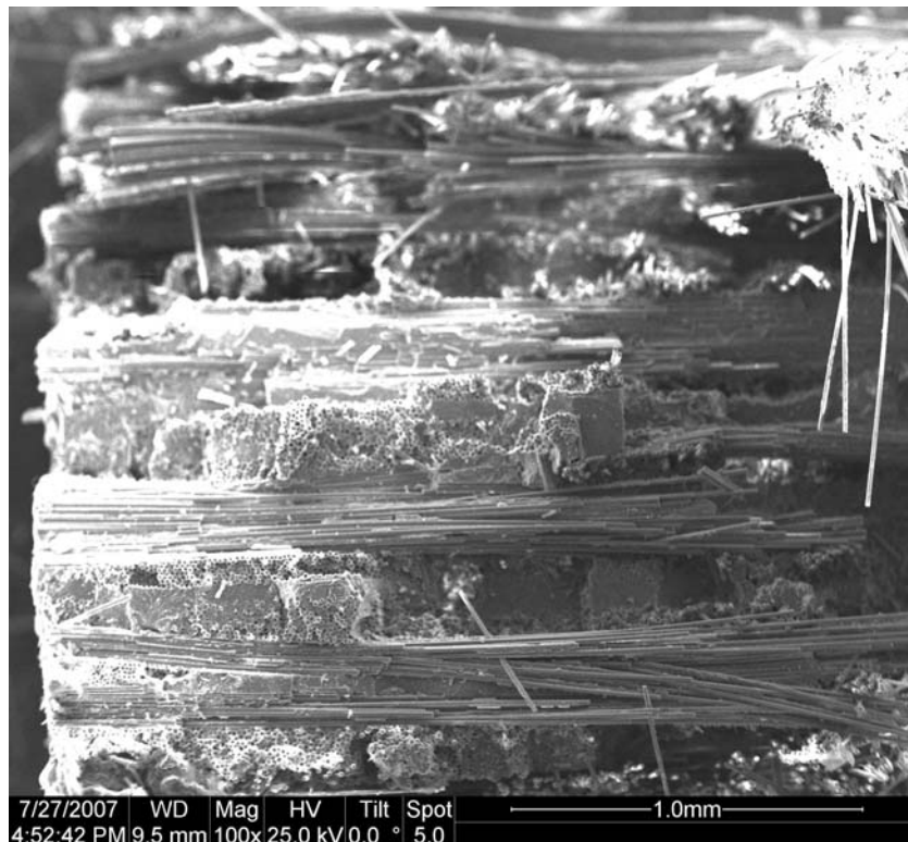
Figure 134. Fracture surface of N720/A specimen tested with cyclic creep-recovery with 1 hour hold times at 100 MPa in steam at 1200 °C.
