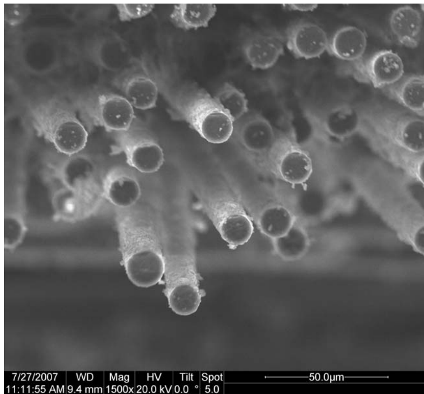
Figure 144. Fracture surface of N720/A specimen tested with cyclic creep-recovery with 1 hour hold times at 100 MPa in steam at 1200 °C, possible kinking.
