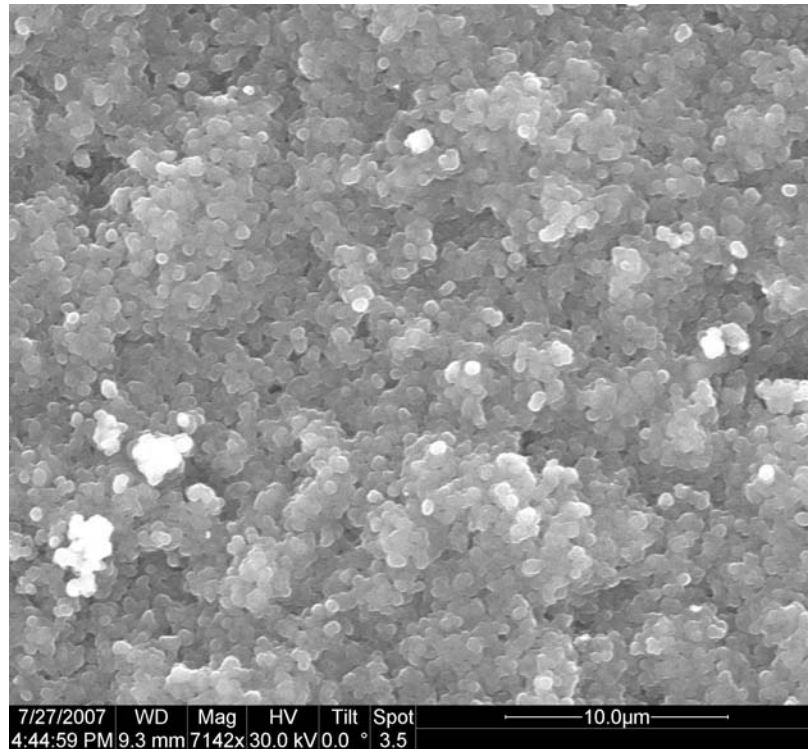
Figure 133. Fracture surface of N720/A specimen tested with cyclic creep-recovery with 1 hour hold times at 100 MPa in steam at 1200 °C.
