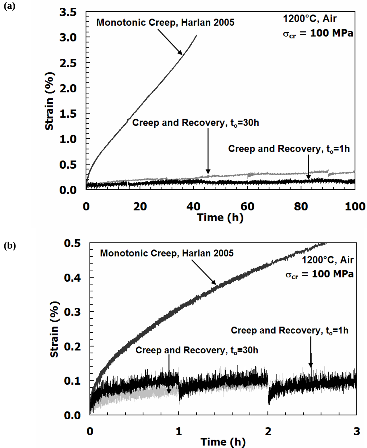
Figure 26. Creep strain vs. time curves for N720/A specimens obtained in cyclic creep tests with \sigma_{max} = 100 \text{ MPa} and t_0 = 1 \text{ h} and 30 \text{ h} conducted at 1200^\circ \text{C} in laboratory air. Monotonic creep data at 100 \text{ MPa} from Harlan [14] are also shown. (a) Time scale chosen to show up to 100 \text{ h} of creep and (b) time scale reduced to clearly show creep curves produced during individual cycles.
