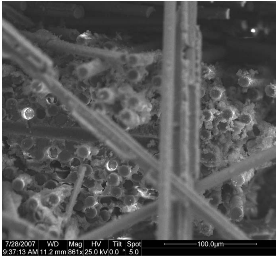
Figure 163. Fracture surface of N720/A specimen tested with cyclic creep-recovery with 0.05 hour hold times at 125 MPa in steam at 1200 °C.
