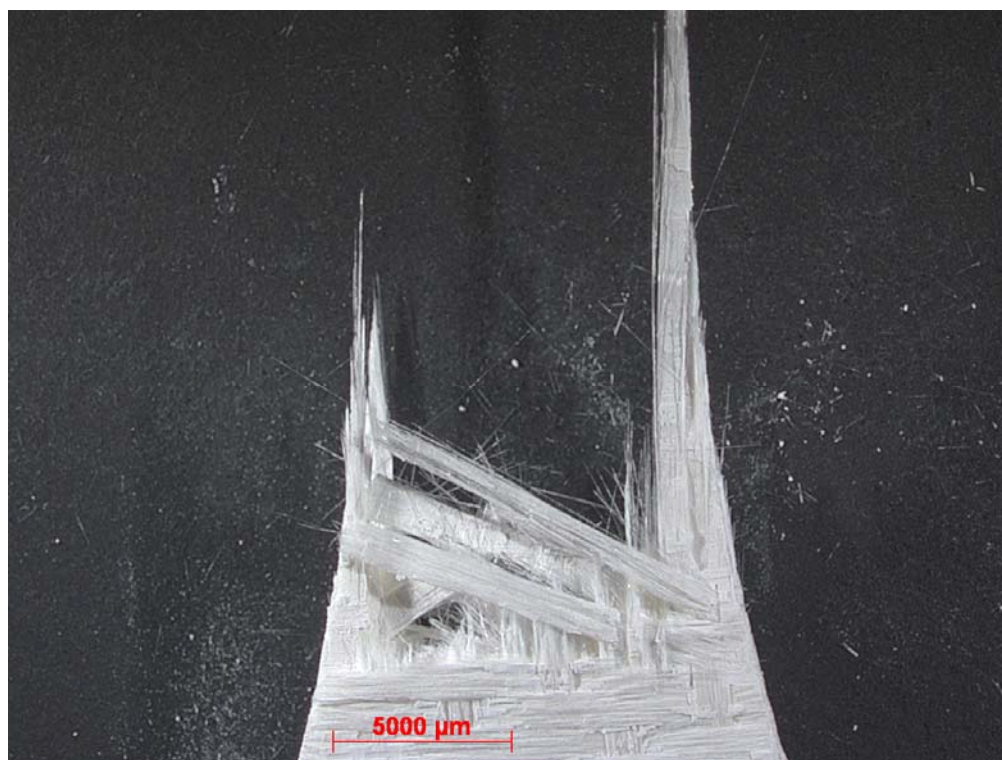
Figure 68. Fracture surface of N720/A specimen tested with cyclic creep-recovery with 1 hour hold times at 125 MPa in air at 1200 °C.
