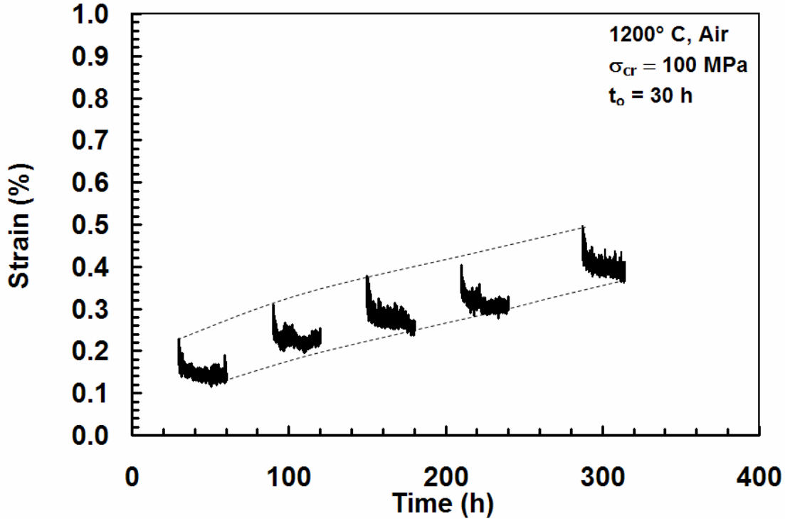
Figure 31. Strain vs. time curves for N720/A composite obtained during recovery periods of cyclic creep test with \sigma_{max} = 100 \text{ MPa} and t_0 = 30 \text{ h} conducted at 1200^\circ \text{C} in laboratory air. Similar amounts of strain are recovered during each cycle.
