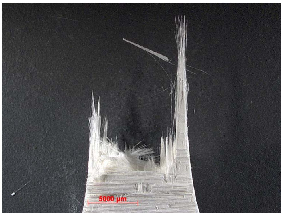
Figure 60. Fracture surface of N720/A specimen tested with cyclic creep-recovery with 1 hour hold times at 100 MPa in air at 1200 °C.
