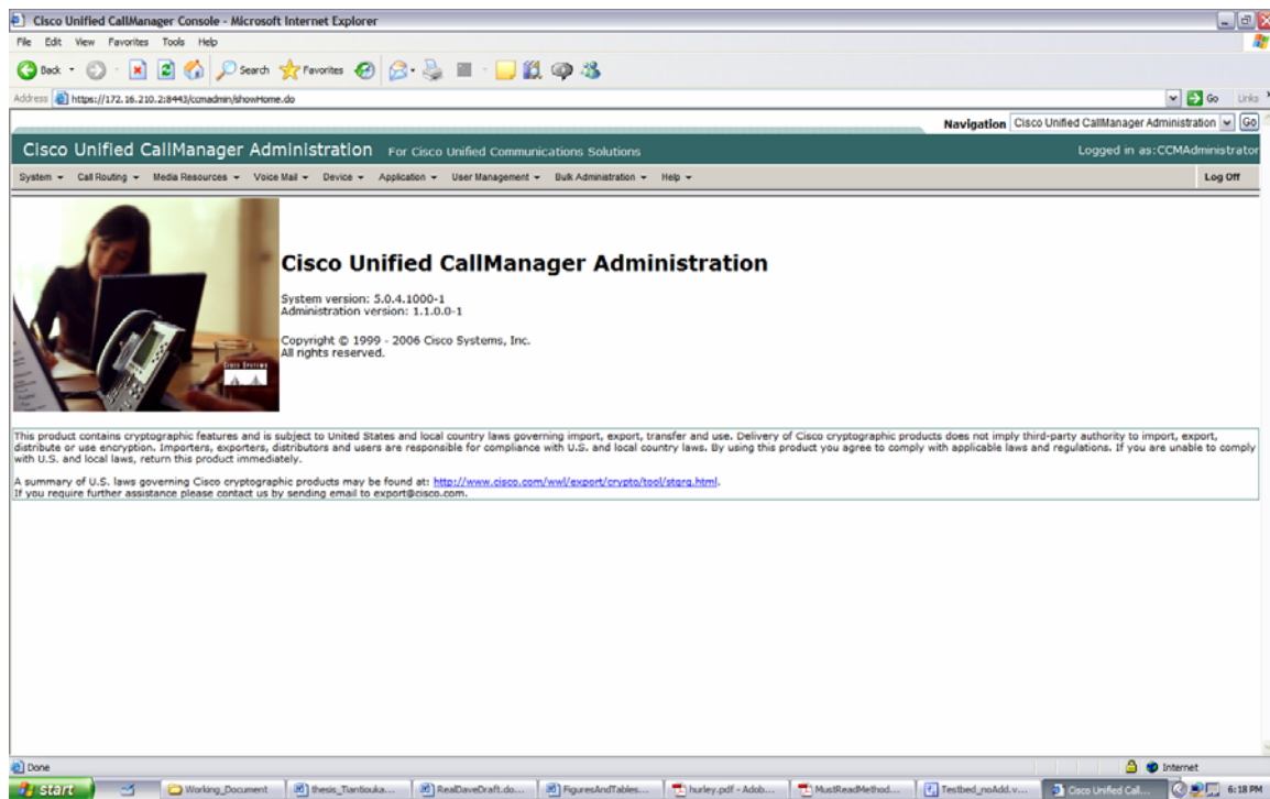
Figure 53. CallManager Login
