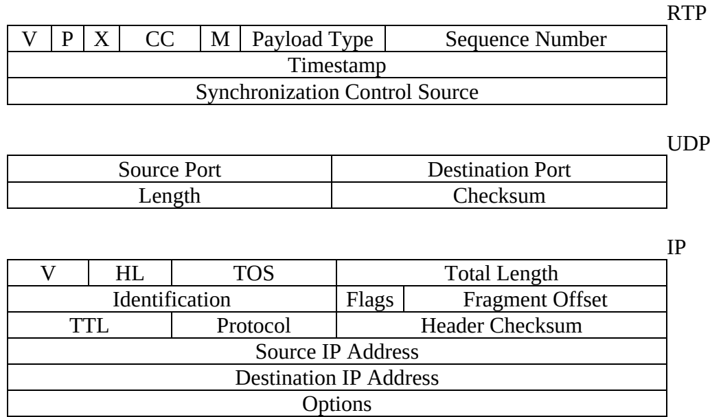
Figure 10. RTP-UDP-IP Headers
