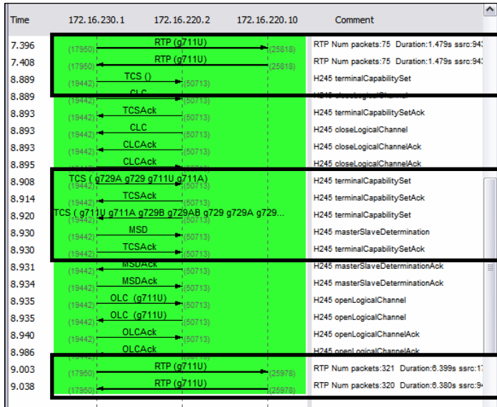
Figure 28. Message Flow During Hold Initiation
