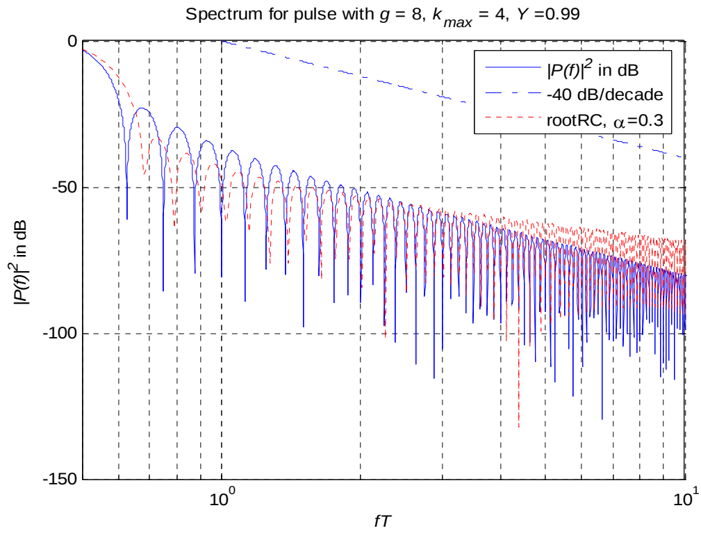
Figure 20 Comparison of duration 8T , new (with k_{\max} = 4 and Y = 0.99 ) and truncated root raised cosine (with \alpha = 0.3 ) pulse shapes.
