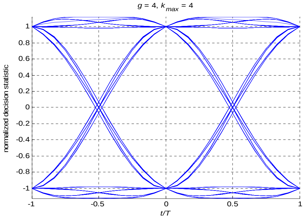
Figure 16 Eye diagram of waveform at the matched filter output for system using the new pulse with duration 4T .
