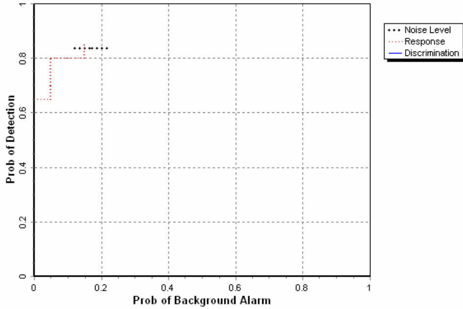
Figure 3. EM/pushcart blind grid probability of detection for response and discrimination stages versus their respective probability of background alarm over all ordnance categories combined.
