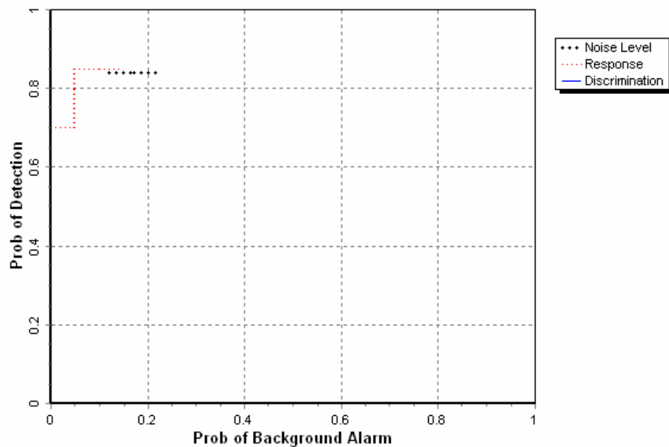
Figure 5. EM/pushcart blind grid probability of detection for response and discrimination stages versus their respective probabilities of background alarm for all ordnance larger than 20 mm.
