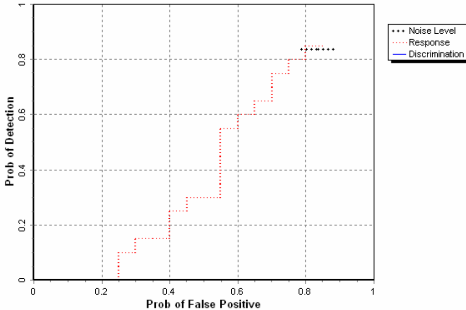
Figure 2. EM/pushcart blind grid probability of detection for response and discrimination stages versus their respective probability of false positive over all ordnance categories combined.
