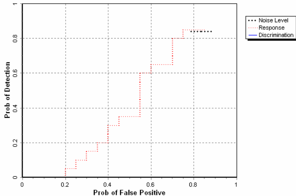
Figure 4. EM/pushcart blind grid probability of detection for response and discrimination stages versus their respective probability of false positive for all ordnance larger than 20 mm.
