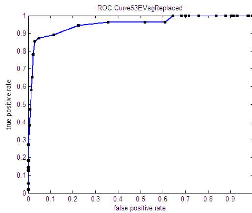
Figure 54. ROC curve for G channel replacement using 53 eigenvectors.
