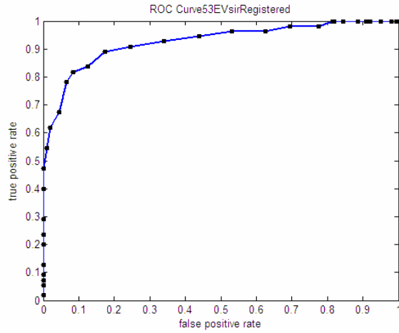
Figure 58. ROC curve for IR based on 53 eigenvectors.
