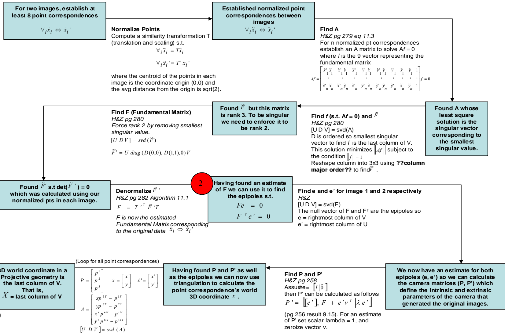
Figure 10. Projective Reconstruction Flow Chart.
