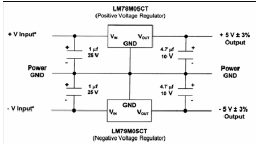
Figure 43. BEI Recommended Voltage Regulator Circuit.
