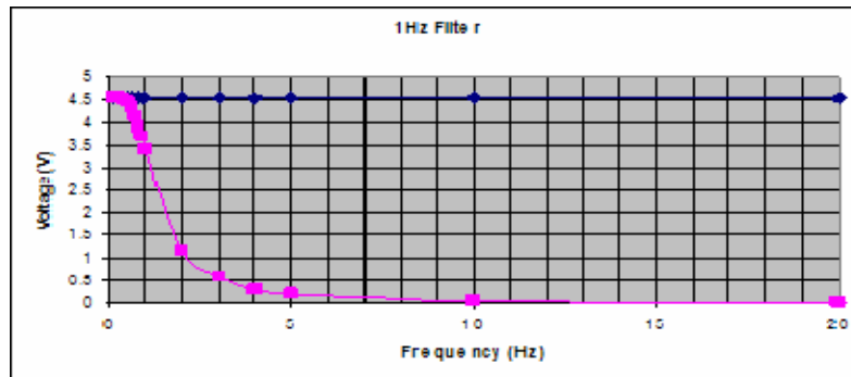
Figure 50. Voltage Input vs. Filtered Input.
