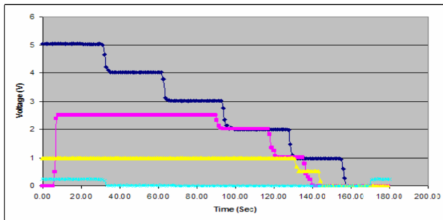
Figure 23. Clipping vs. Gain.
