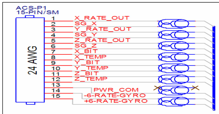
Figure 4: 15-Pin Connector
