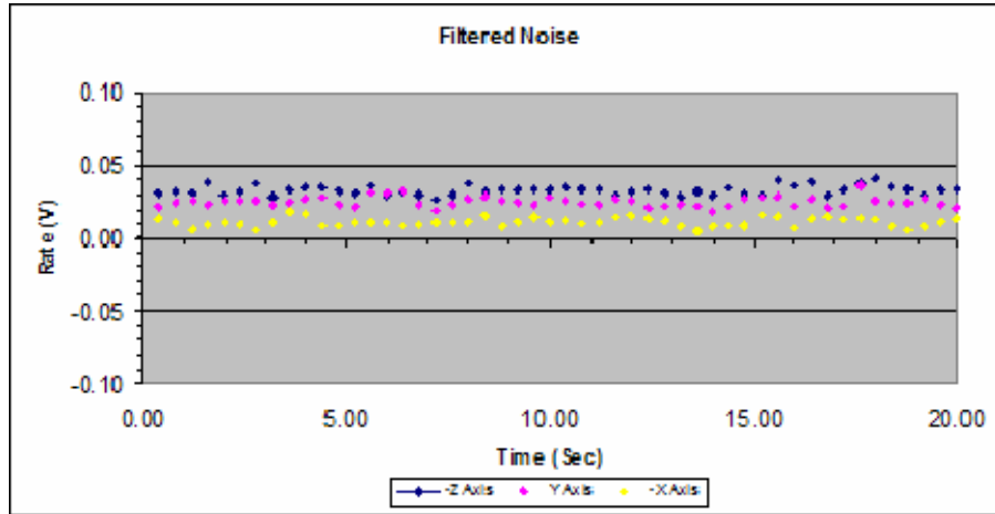
Figure 68. MEMS 3-Axis Rate Output.
