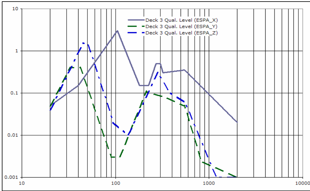
Figure 3. Deck Three Launch Profile (Vibrational).
