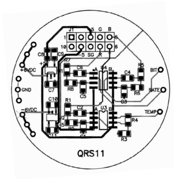
Figure 59. MEMS PCFB Final CAD Diagram.
