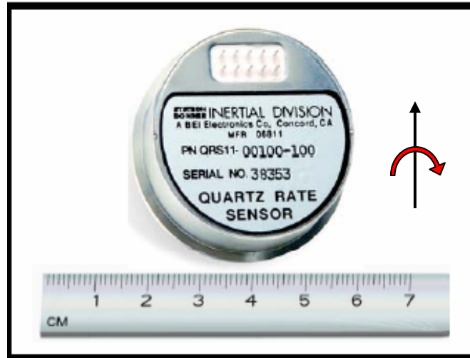
Figure 4. QRS11 Sensor.
