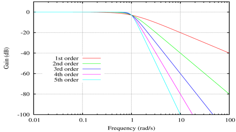
Figure 52. Theoretical Filter Response.
