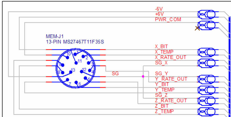
Figure 6: 13-Pin Connector
