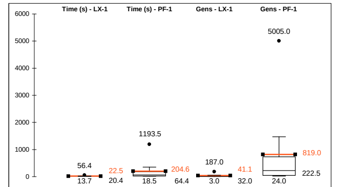
Figure 3: Comparison of Lex and Pareto-based for Test 1
