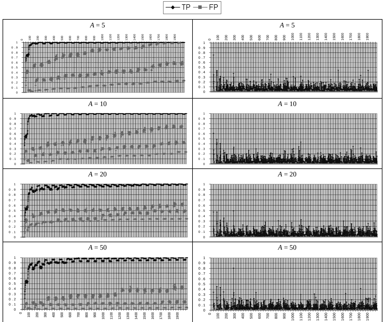
Figure 1. TP and FP rates when A varies and T = 30 , L = 10 , N = 30
