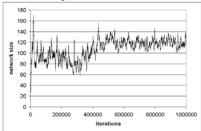
Figure 6: Size evolution of the network running on the trivial data set with introduction of second cluster at 250,000 iterations.
