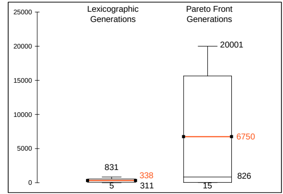
Figure 8: Comparison of Generations for Lexicographic and Pareto-based Queso Scan Test
