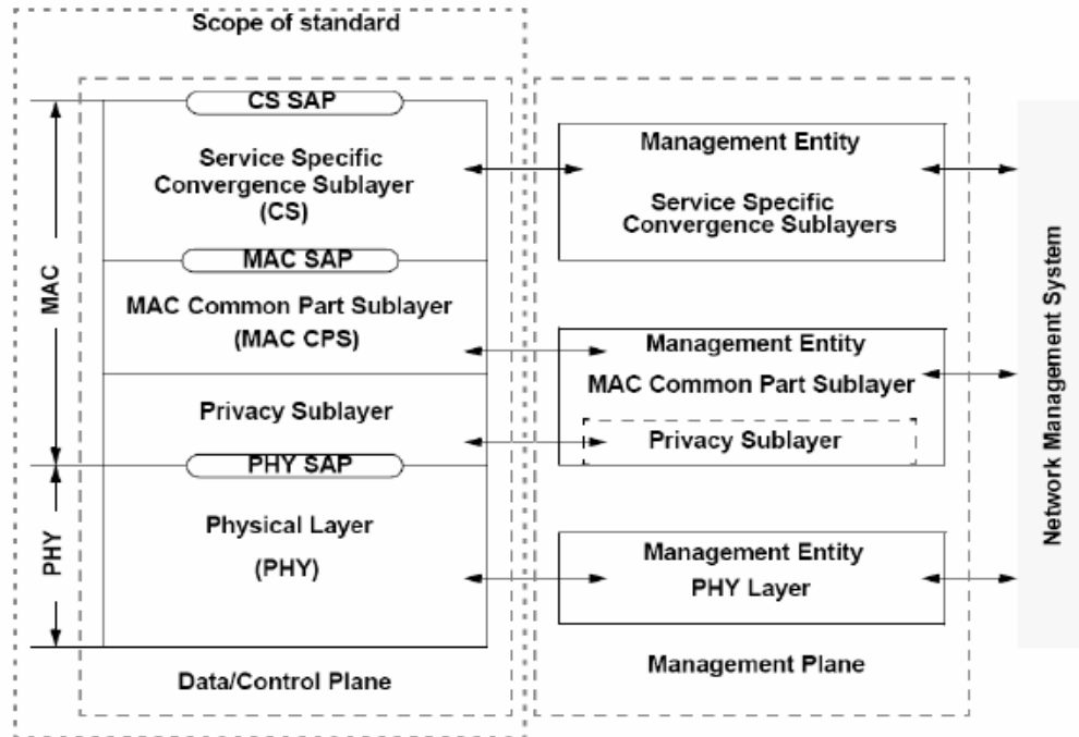
Figure 15. Protocol Layering of 802.16 (From: [11]).
