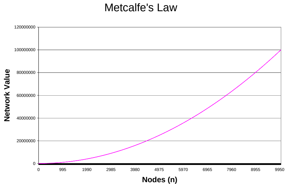
Figure 1 Metcalfe's Law.
