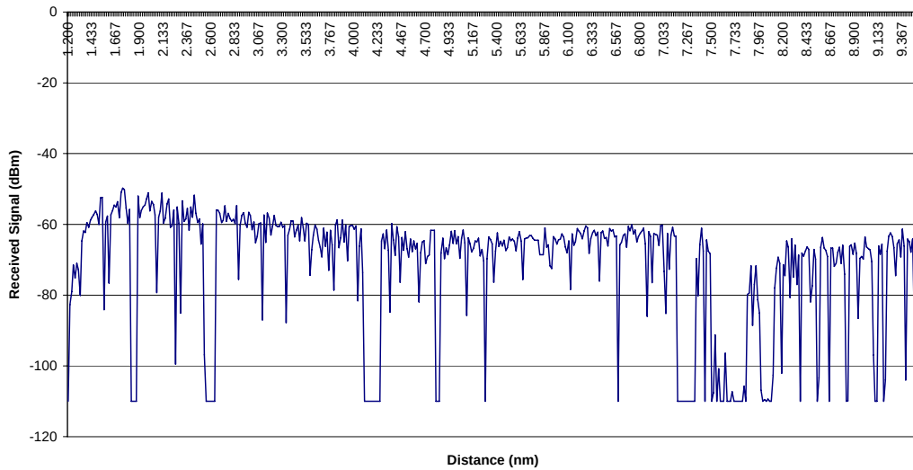
Figure 41 TNT 07-02 Motorola PTP 600 Received Signal (Inbound Leg).
