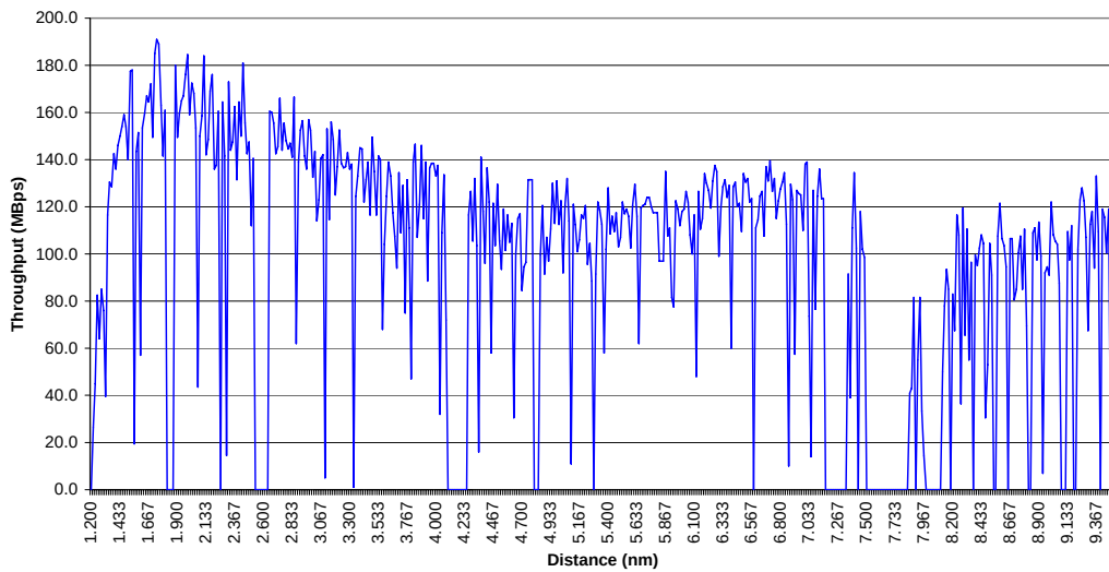
Figure 42 TNT 07-02 Motorola PTP 600 SNMP Throughout (Inbound Leg).
