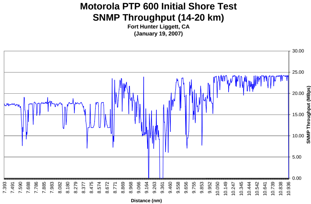
Figure 32 Motorola PTP 600 FHL SNMP Reported Throughput (14-20 km).
