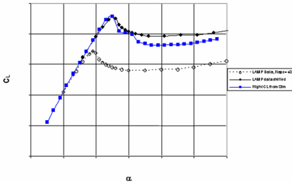
Figure 20. – Comparison of 1/12-scale business jet model lift coefficient at flaps = 40 measured in the LAMP wind tunnel with flight lift coefficient represented by the manufacturer's simulation model shifted to flight C_{L_{max}}
