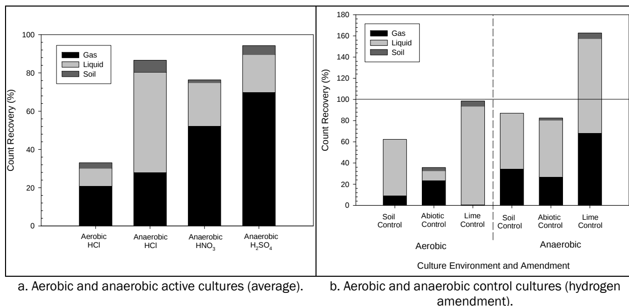
Figure 12. Activity balance of RDX following alkaline hydrolysis at pH 10.5 and incubation with soil.
