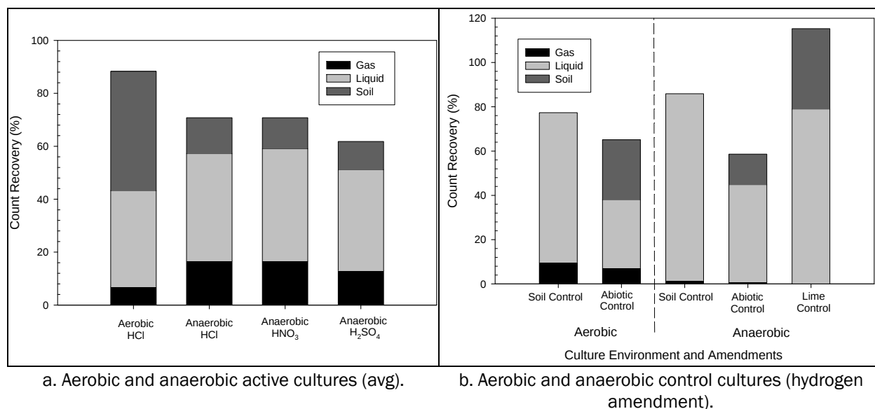
Figure 6. Activity balance of TNT following alkaline hydrolysis at pH 12.5 and incubation with soil.
