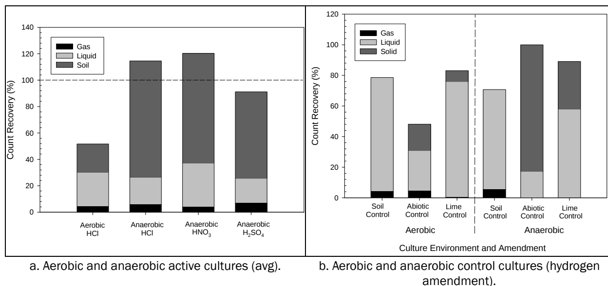
Figure 8. Activity balance of TNT following alkaline hydrolysis at pH 10.5 and incubation with soil.
