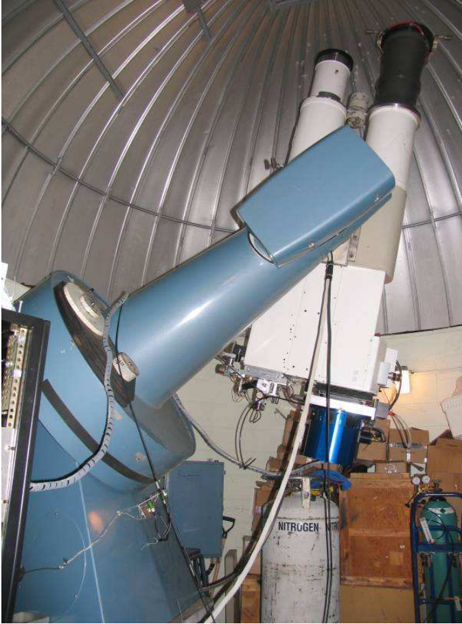
Figure 2. 10k camera with a single STA1600 chip mounted at the USNO astrograph, currently located at the Flagstaff station.
