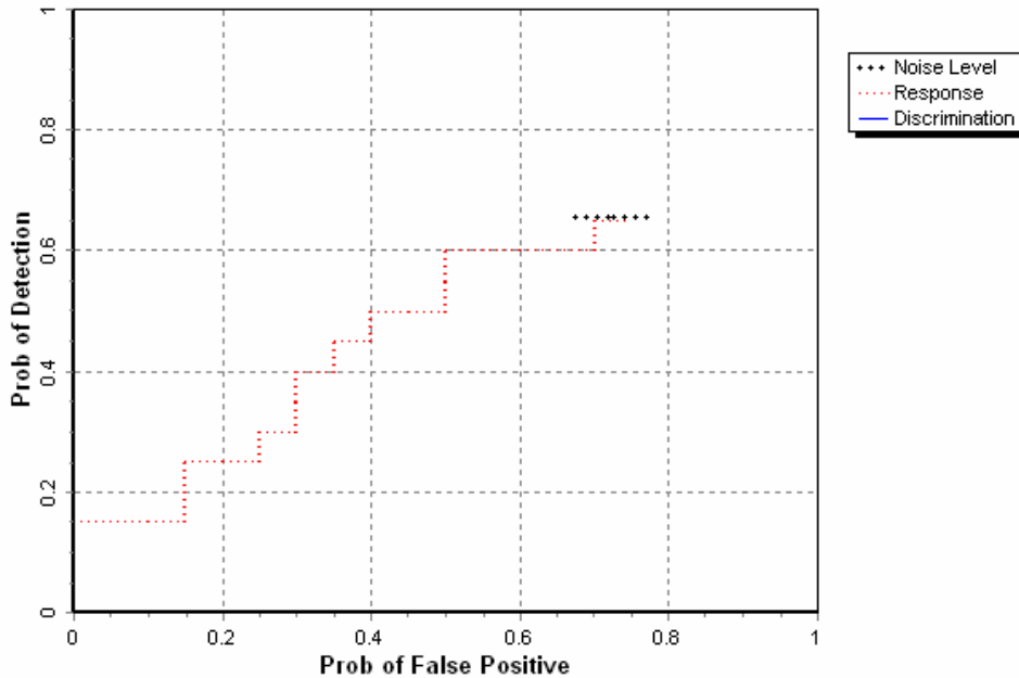
Figure 2. EM/pushcart mine grid probability of detection for response and discrimination stages versus their respective probability of false positive over all ordnance categories combined.
