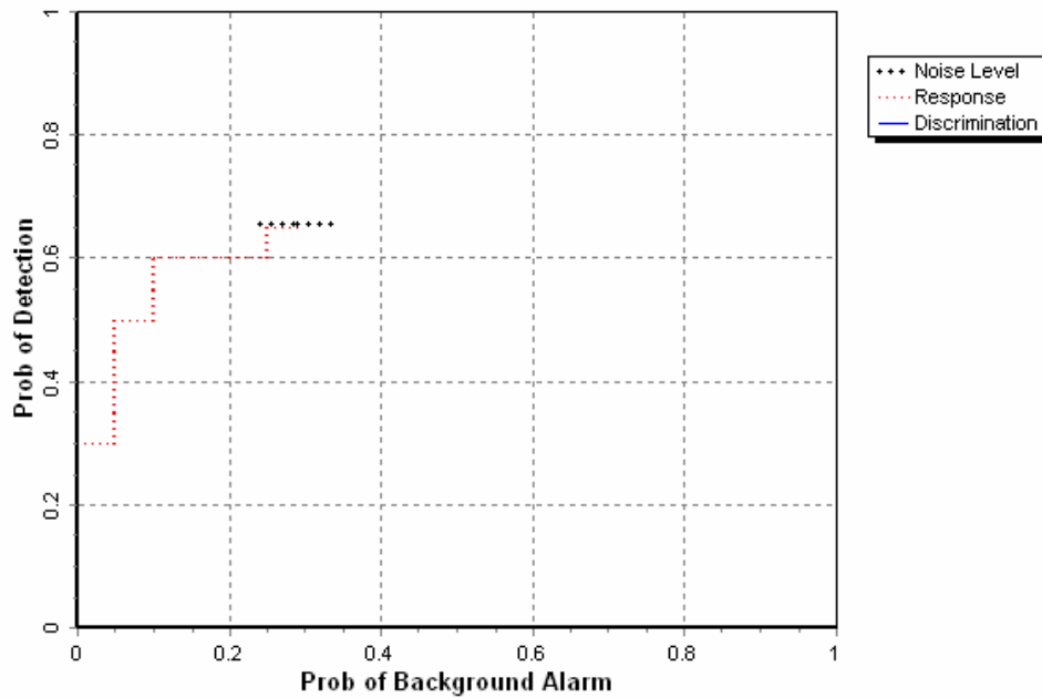
Figure 3. EM/pushcart mine grid probability of detection for response and discrimination stages versus their respective probability of background alarm over all ordnance categories combined.
