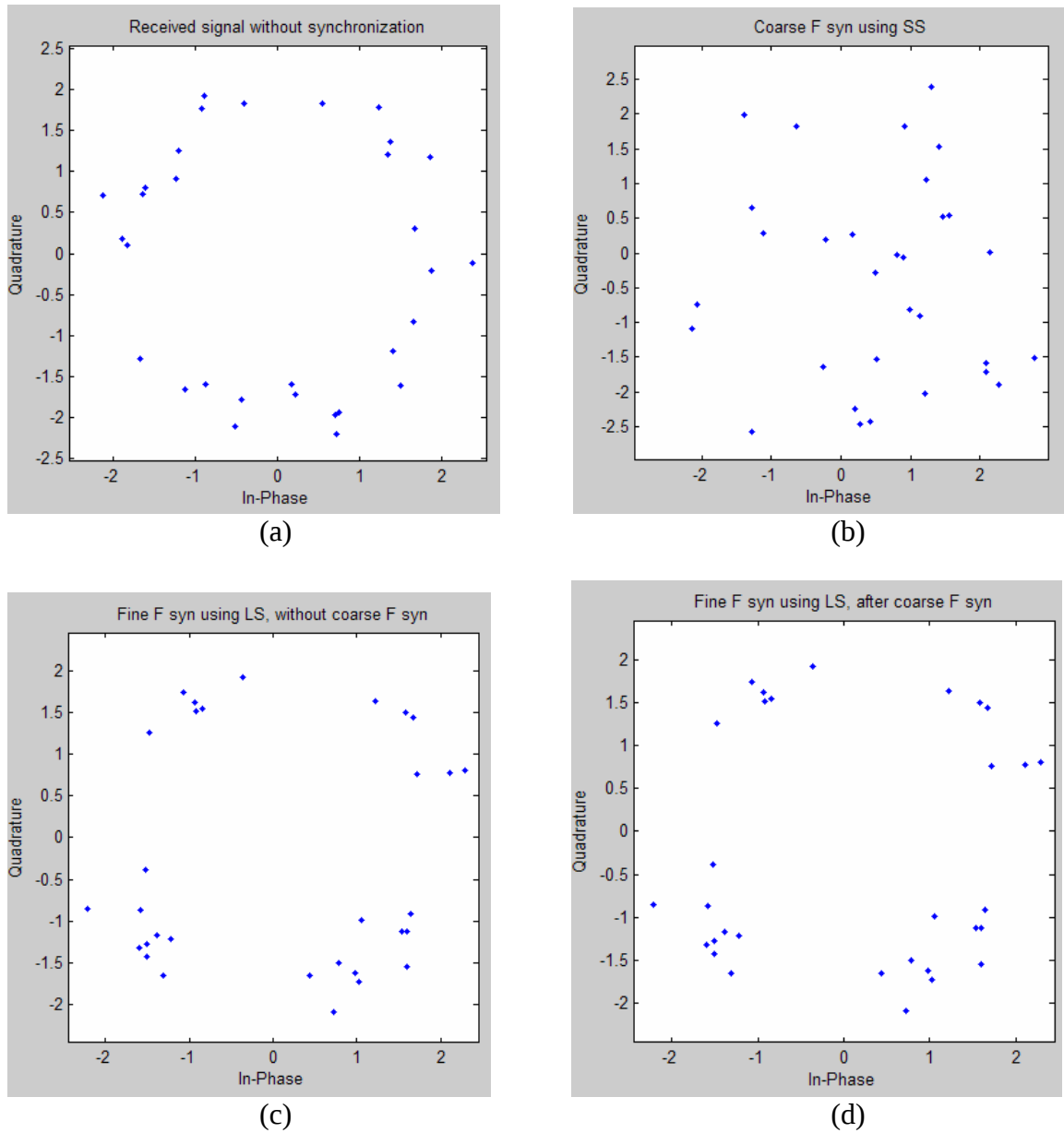
Figure 44. Frequency synchronization effect in Signal 5.
