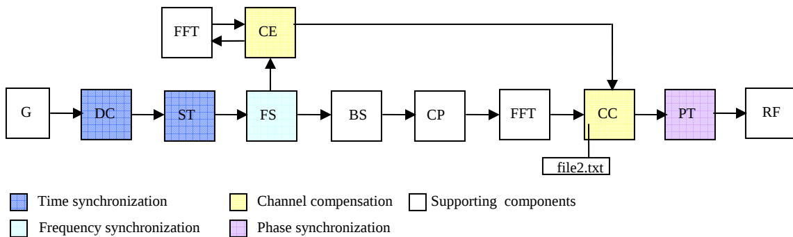
Figure 34. Test 2 waveform.
