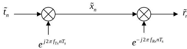
Figure 7. Analytic signal.
