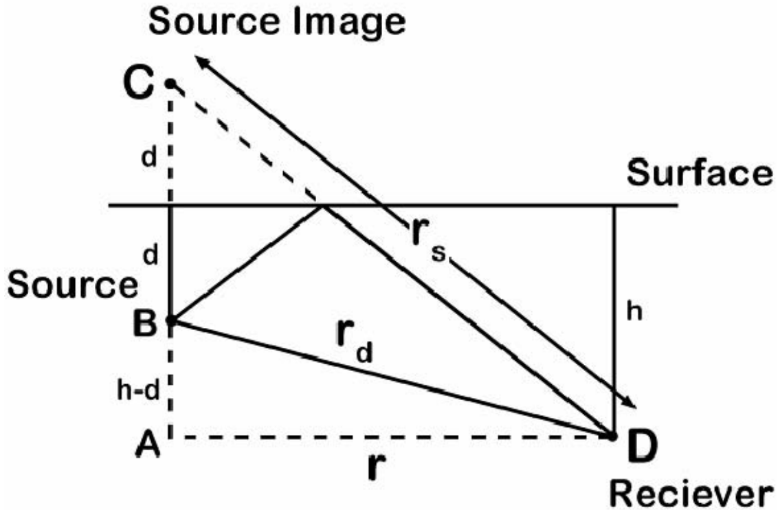
Figure 3. Geometry for analyzing surface interference [From Kapolka, 2007].
