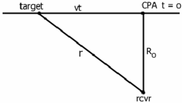
Figure 5. Geometry for analyzing a spectrogram pattern for a target passing through CPA [From Kapolka, 2007].
