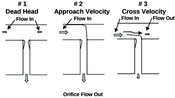
Figure 3 - Orifice Entrance Test Configurations
