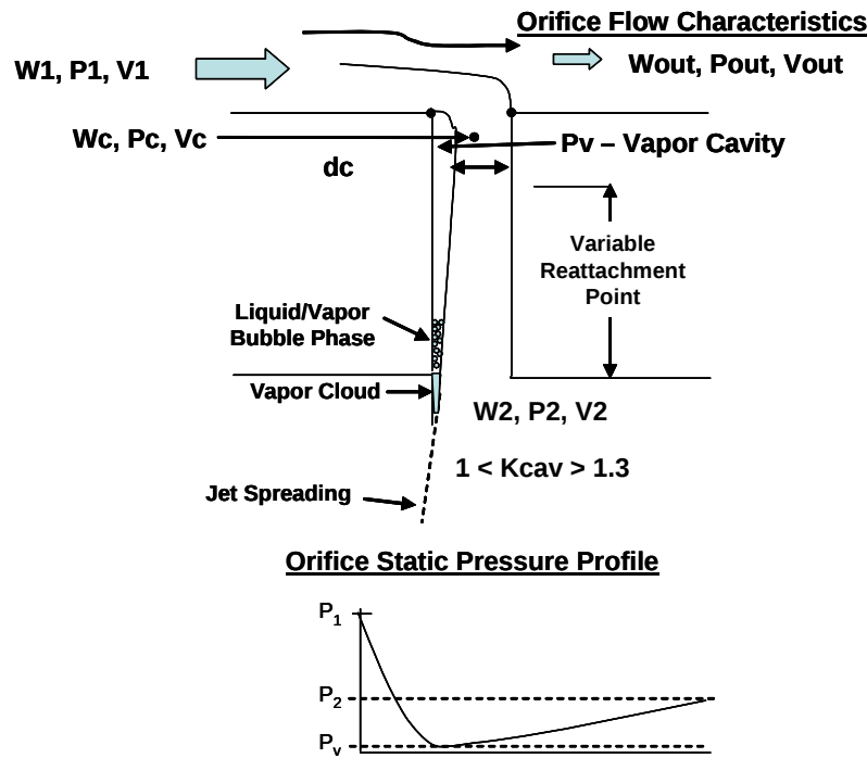
Figure 26 - Illustration of Supercavitation Jet Characteristics
