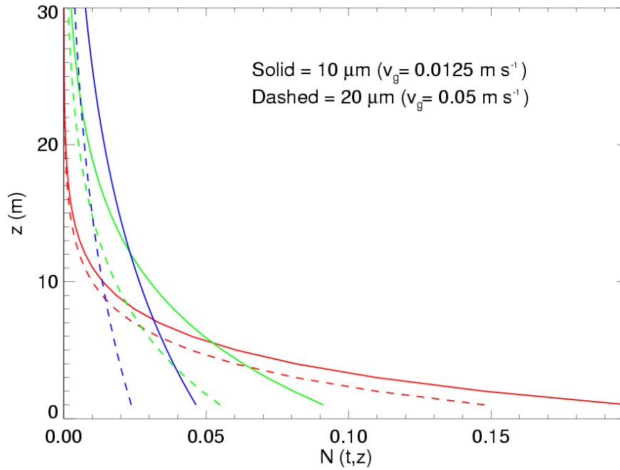
Figure 46. N for a single puff plume with gravitational settling of particles and a capped boundary layer (100 m) at 20, 50, and 100 seconds as calculated from equation 80, as corrected by N_0 as calculated by integrating N/N_0 at time = 0.01 s. Solid lines are for 10 \mu\text{m} particles, dashed lines for 20 \mu\text{m} particles.
