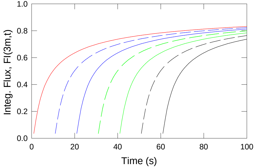
Figure 16. FI(3m,t) for 7 puffs offset by 10 seconds for the perfectly reflecting case. At 70 seconds the sum of the puffs is the same as the sum of the puffs at 60 seconds plus the contribution of the first puff at 70 seconds.
