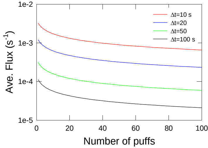
Figure 14. Upward average flux, SI(z, MDx) , at 2 m for puff separations of 10, 20, 50, and 100 seconds as a function of the total number of puffs for an absorbing surface.
