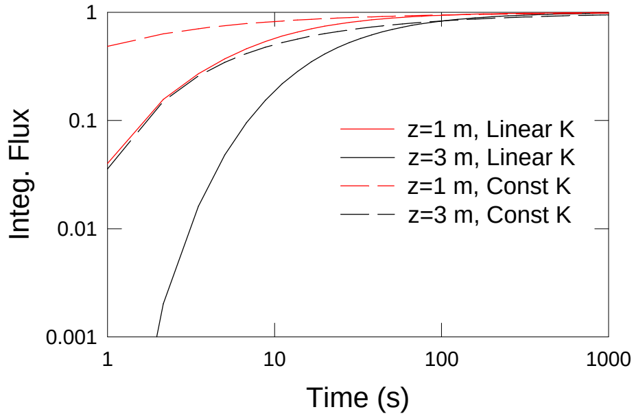
Figure 17. The integrated flux at time \tau at 1m (red) and 3 m (black) from a single puff at z=0.2 m for a perfectly reflecting surface. The solid lines are for linearly increasing diffusion coefficient ( K=0.16z ) and the dashed lines for constant K=1 \text{ m}^2 \text{ s}^{-1} .
