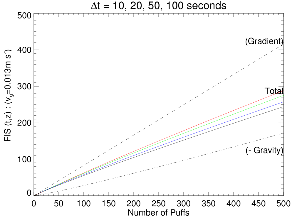
Figure 43. Sum of the integrated puffs as a function of the number of puffs for Dt = 10, 20, 50 and 100 s. The solid lines are the net flux and the broken lines for the gradient and gravitational components for Dt=100 s.
