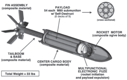
Figure 2.10 XM984 Uses a Rocket Motor to Reach Up to 11 km
