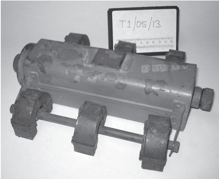
Figure 2.26 Magnetic Limpet Mine
