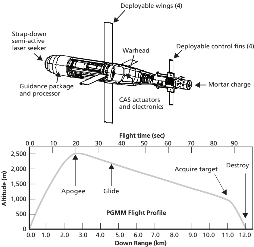
Figure 2.12 The Components and Flight Profile of ATK's PGMM
