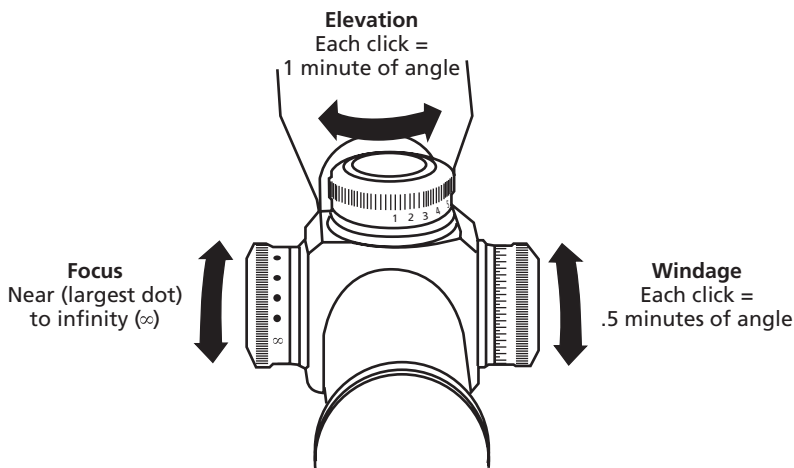
Figure 2.17 A Common Sniper Scope Features Knobs That Allow a Shooter to Adjust for Elevation and Windage
