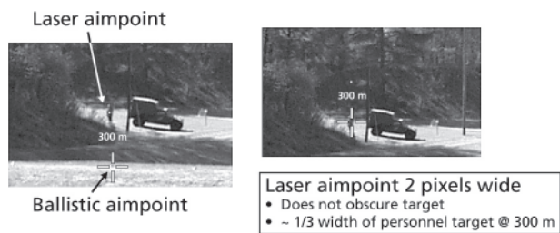
Figure 2.3 XM104 Sighting System and Ballistics Computer in Action
