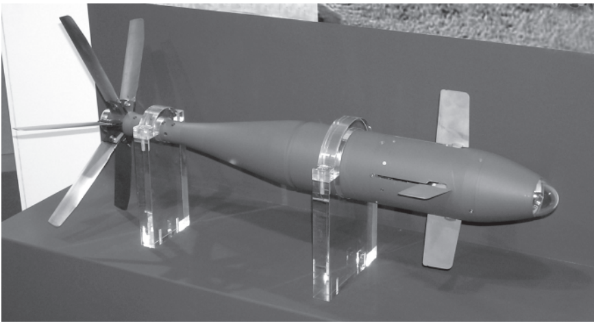
Figure 2.11 Israel Aircraft Industries' Fireball Has Four Deployable Wings as Do the PGMM and Armement Léger à Fibre Optique (ALFO)
