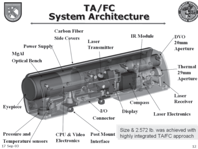
Figure 2.2 Components of the XM104 TA/FC for Use with the XM25
