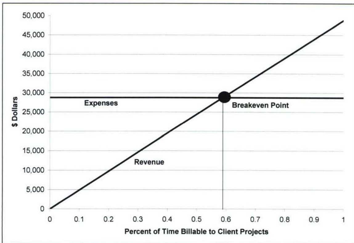
Figure 8: Breakeven Analysis
