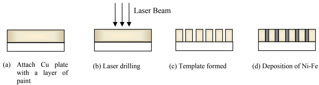
Fig. 10. An outline of the process sequence to fabricate Ni-Fe micro-pillars arrays using laser micro-machining and electrodeposition.
