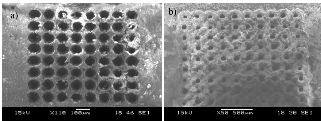
Fig. 19. (a) Template fabricated using UV laser; (b) template fabricated using Green laser.
