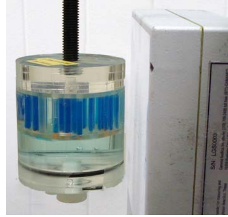
Fig. 2. Contrast-detail phantom in water filled cylinder imaged using a simple circular scan at a close radius of rotation. Blue food coloring was added to the fluid inside the tubes for better visibility.
