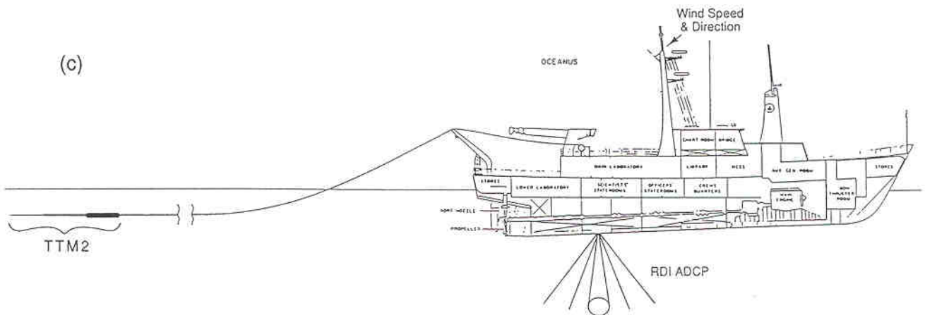
Figure 2. TTM2 tow body and towing configuration. (a) Tow body in cradle. (b) Jim Osse holding tow body. (c) Sketch of towing configuration during OC216.
