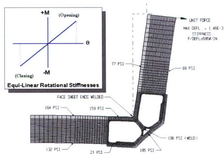
Figure 32. Equilinear Rotational Stiffnesses: Opening Versus Closing Moments for D-Extrusion Joints
