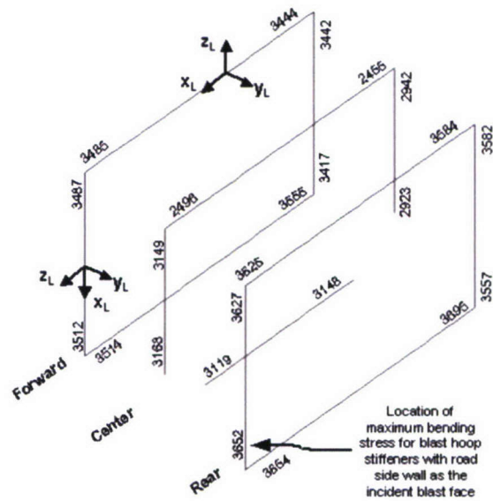
Figure 100. Blast Hoop Stiffener Beam Elements and Local Coordinate Systems
