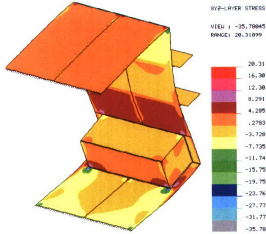
Figure 26. Contour Plot of Honeycomb Core Transverse Shear Stress \sigma_{yz} for Section Test
