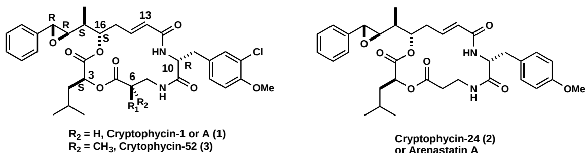
Fig. 1: Structures of cryptophycins
