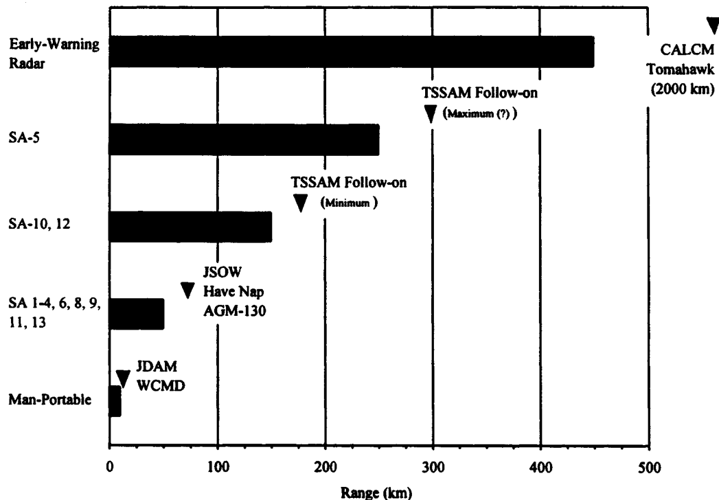
FIGURE 5. RANGES OF STANDOFF WEAPONS AND LIKELY ENEMY-HELD SAMs
