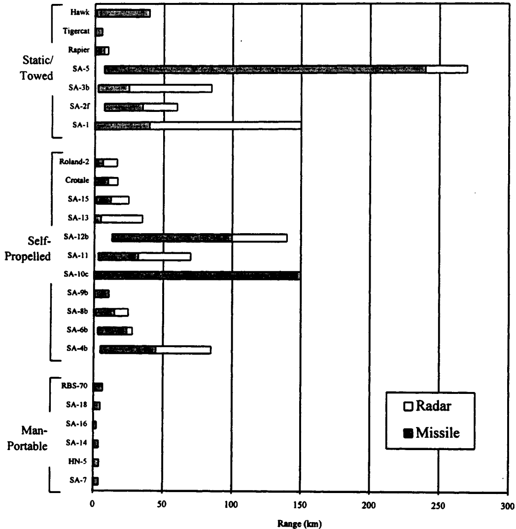
FIGURE 4. RANGES OF LIKELY ENEMY SAMs AND THEIR ASSOCIATED ENGAGEMENT RADARS
