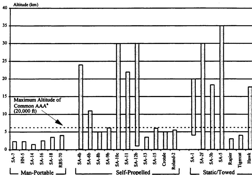
FIGURE 2. OPERATING ALTITUDES OF LIKELY ENEMY SAMs
