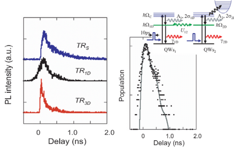
Fig. 7. TR_S , TR_{1D} , and TR_{3D} show TRNFPL signal obtained at I_S , I_{1D} , and I_{3D} , respectively (left). Theoretical results on the transient exciton population dynamics (solid curves) and experimental PL data (filled squares) of 1-DQWs (same as curve TR_{1D} ).
