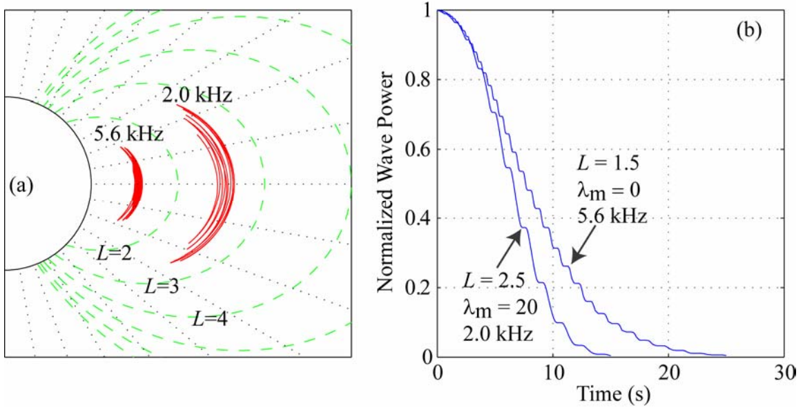
Figure 1: (a) Ray paths of a 5.6- kHz signal injected at L = 1.5 at the equator and a 2.0- kHz signal injected at L = 2.5 and \lambda = 20^\circ . (b) Variations of the wave power density along the ray paths at different L -shells.
