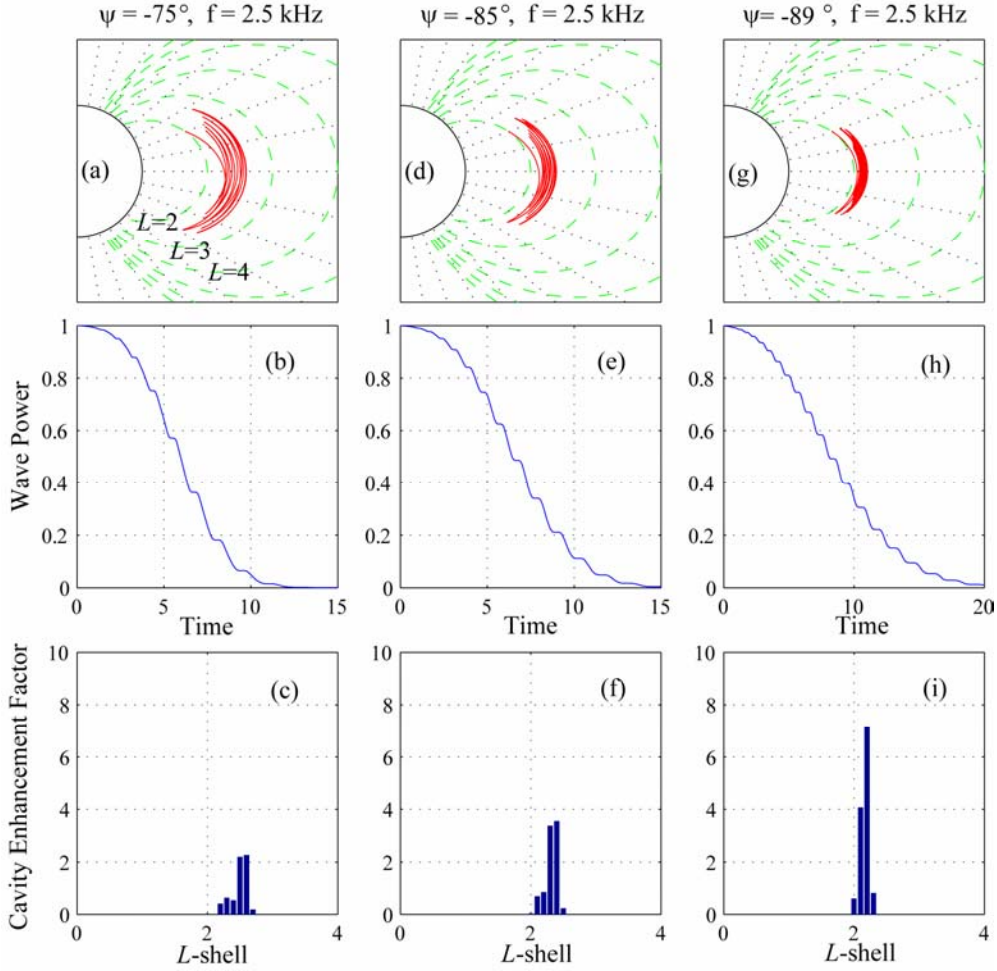
Figure 8: (a) – (i) Similar to before, with parameters indicated on plots. All rays were injected at L = 2 at \lambda = 20^\circ .
