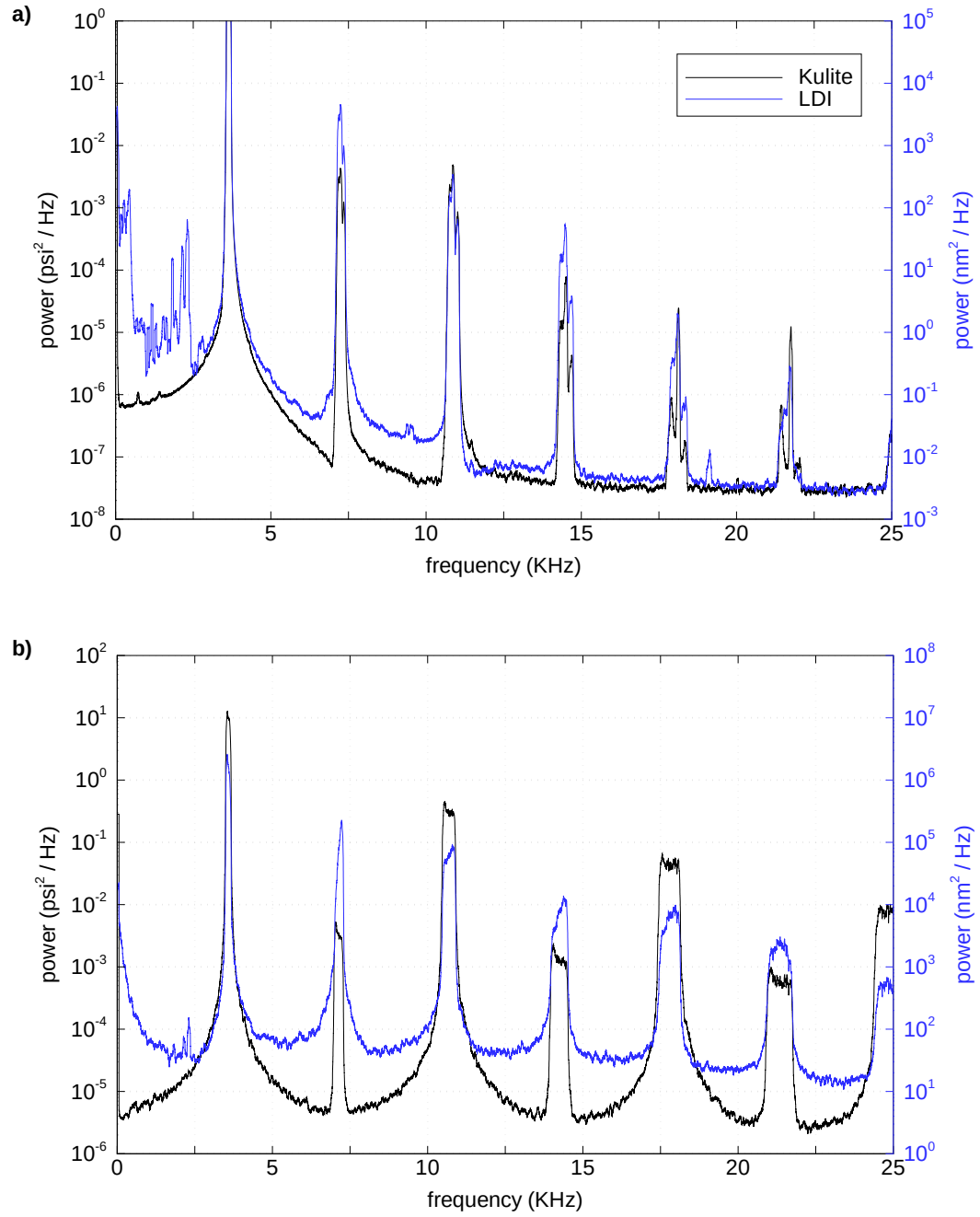
Figure 4.16: Power spectra of forward-facing cavity Kulite and LDI at cavity depth \frac{L}{D} = 2.0 D (before nozzle repolish): a) p_{0,i} = 8 \text{ psi} , b) p_{0,i} = 24 \text{ psi}
