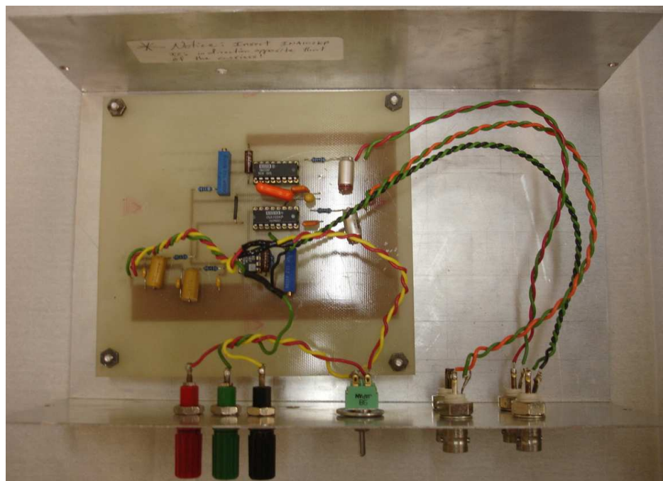
Figure B.25: Kulite box
