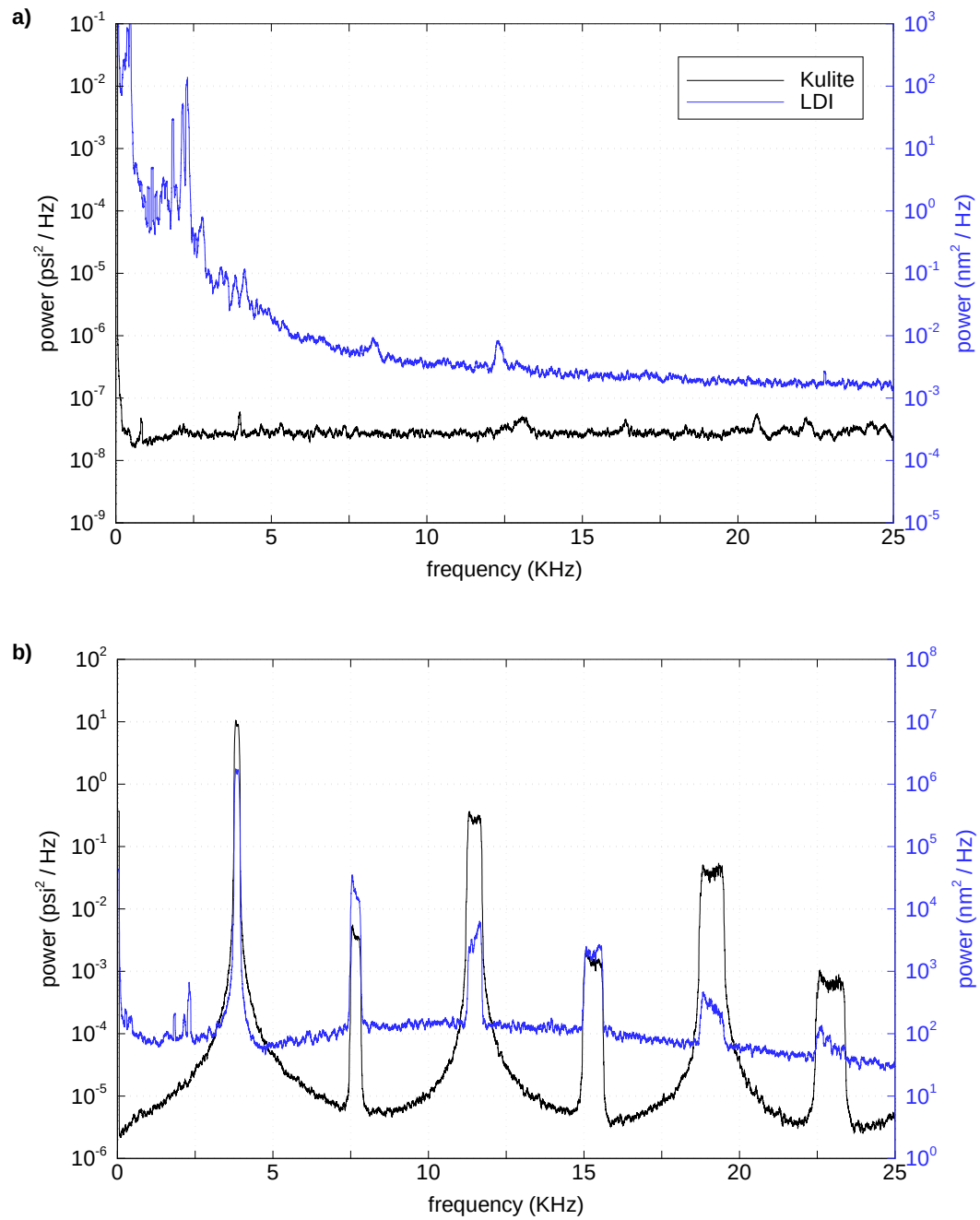
Figure 4.15: Power spectra of forward-facing cavity Kulite and LDI at cavity depth \frac{L}{D} = 1.86 D (before nozzle repolish): a) p_{0,i} = 8 psi, b) p_{0,i} = 24 psi
