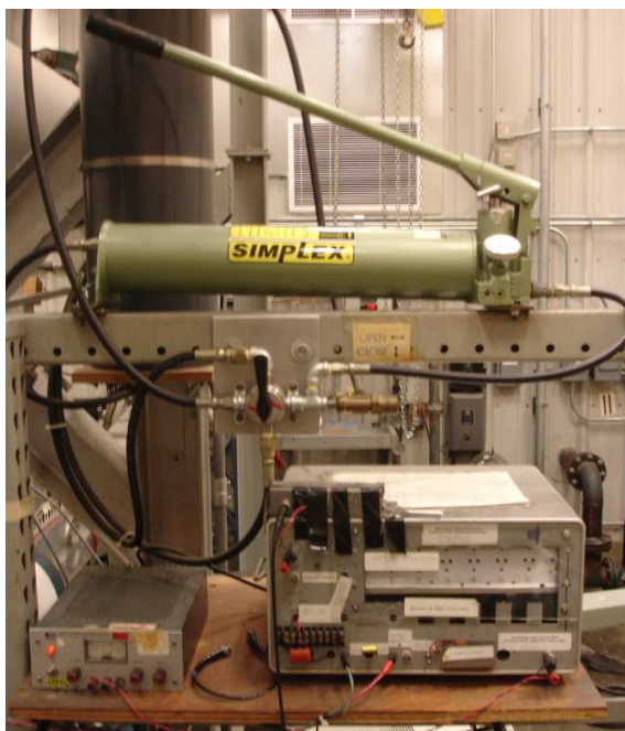
Figure B.9: PQFLT facility, sliding sleeve controls and diaphragm burst electronics
