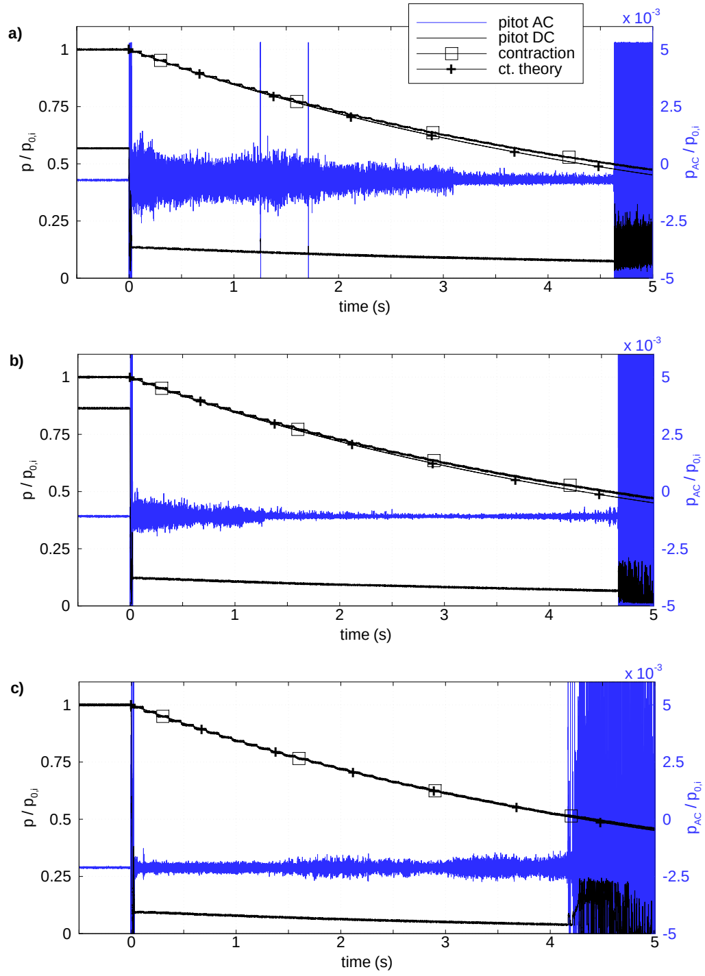
Figure 2.8: Typical pitot and contraction pressure traces: a) p_{0,i} = 24 psi, b) p_{0,i} = 16 psi, c) p_{0,i} = 8 psi
