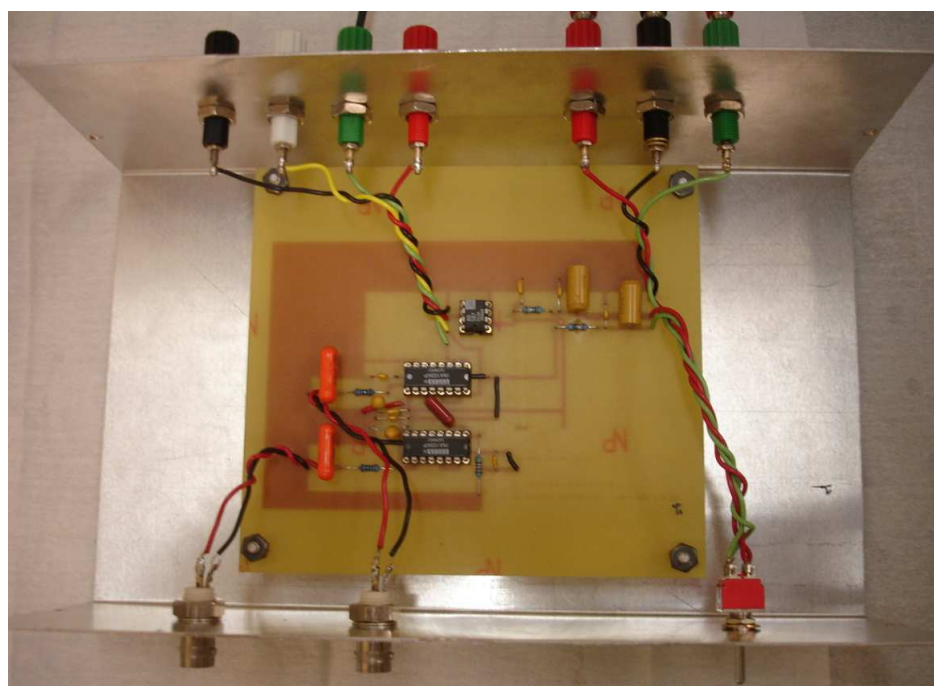
Figure B.26: Constant current anemometer
