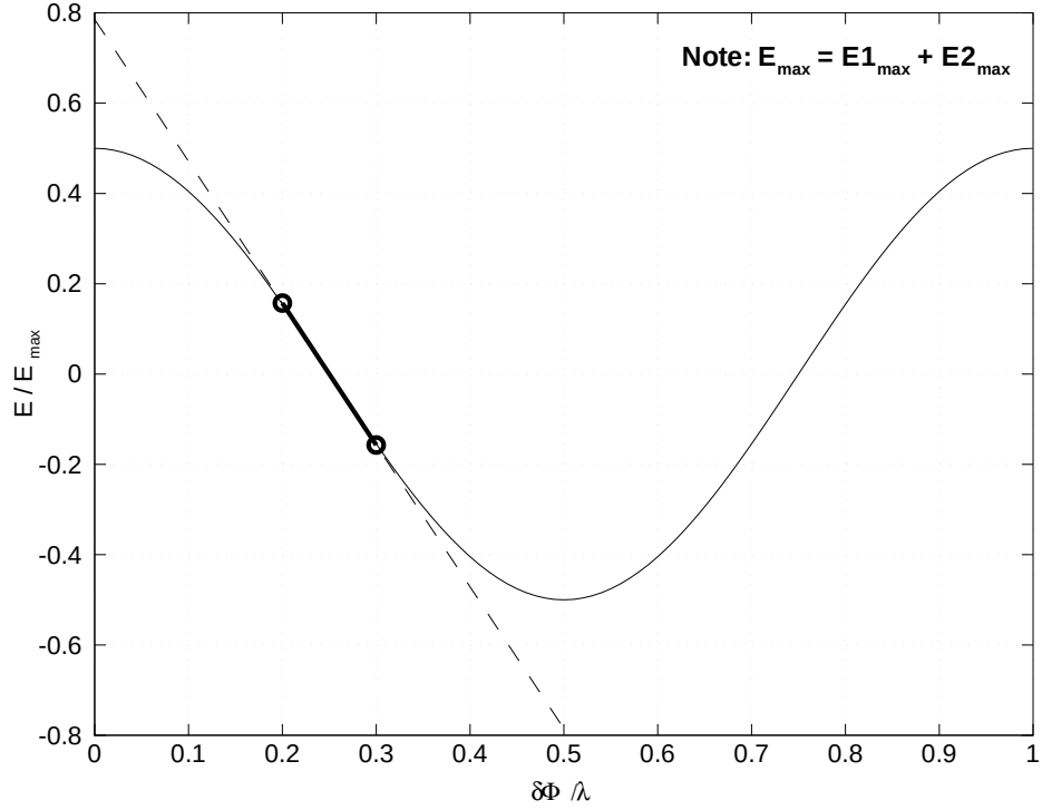
Figure 3.10: Interference slope for differenced photodiodes
