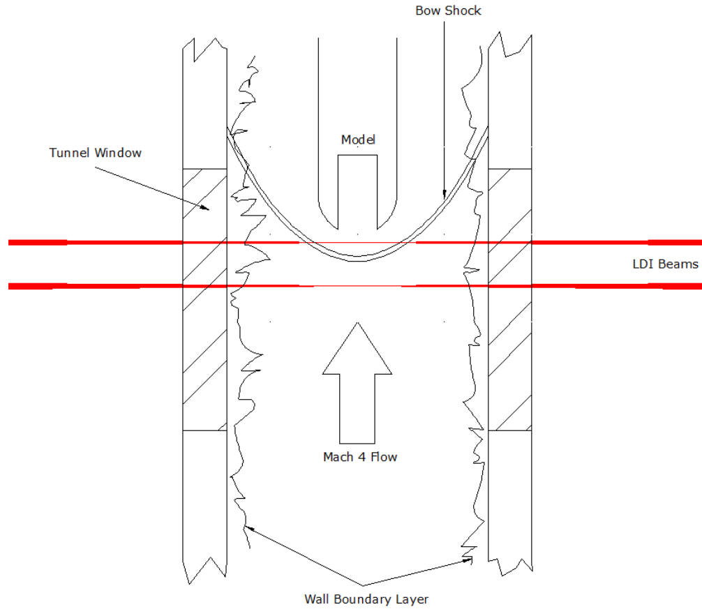
Figure 3.7: Schematic of LDI integration path
