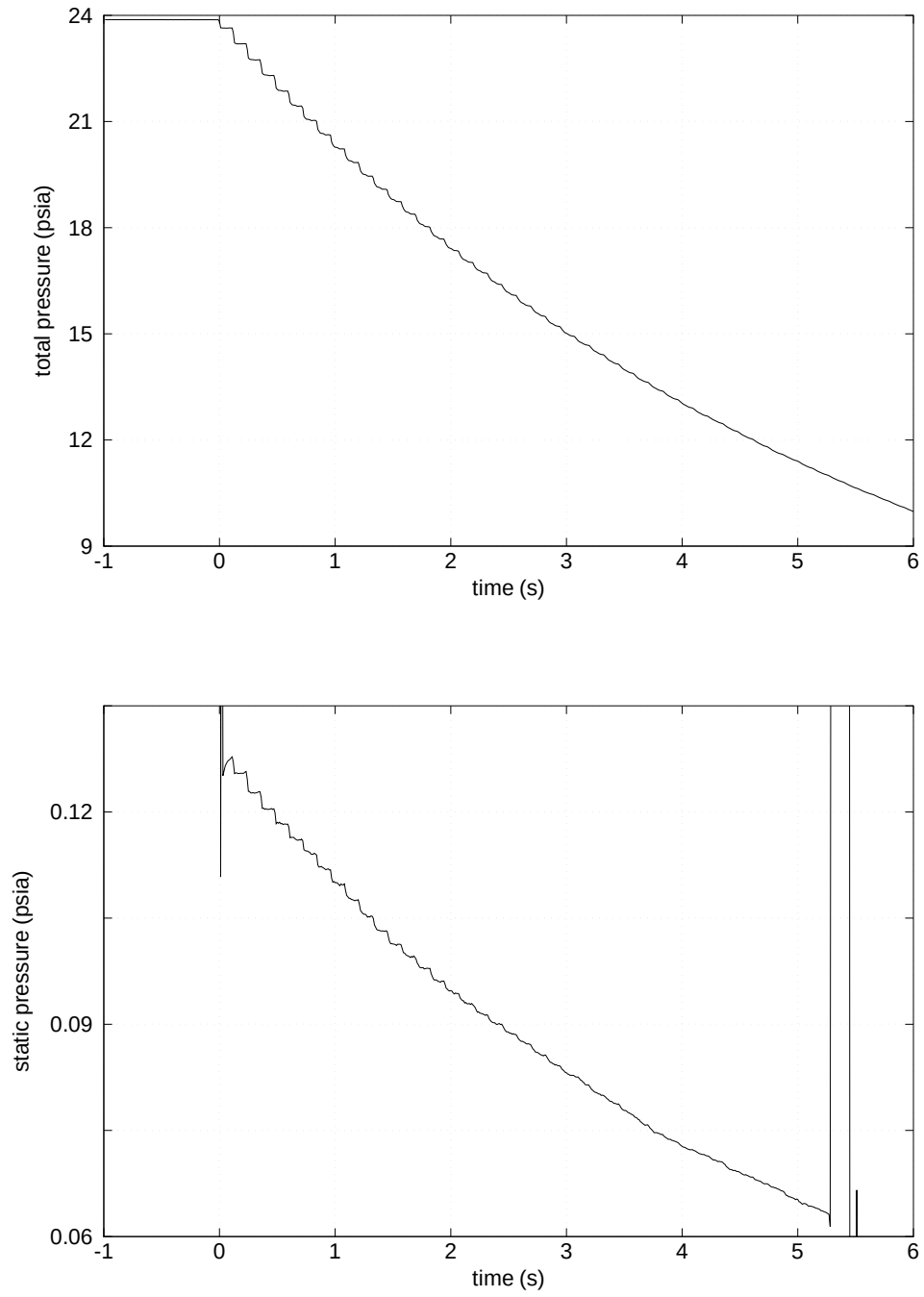
Figure 2.15: Pressure drop throughout tunnel run before repolishing the nozzle.
