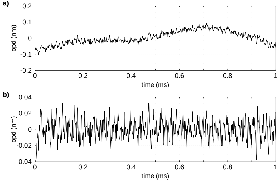
Figure 3.16: LDI electrical noise in the BAM6QT without vibration control: a) raw noise trace, b) raw signal minus running average
