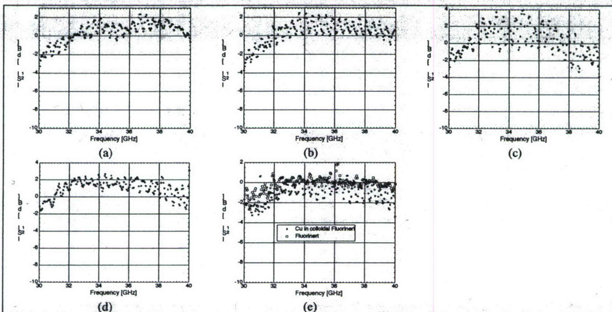
Figure 4. Measured results of the magnitude of the transmission response of (a) 4 mg/ml nano-magnetic particles ( \text{Fe}_3\text{O}_4 ) in Fluorinert, (b) 1 mg/ml nano-magnetic particles ( \text{Fe}_3\text{O}_4 ), (c) 4% v/v nano-Nickel particles in Fluorinert, (d) 10% v/v nano-Cu particles in Fluorinert, and (e) Cu particles in colloidal Fluorinert and unmodified Fluorinert.
