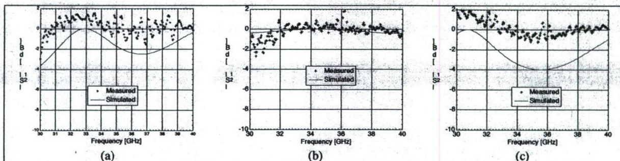
Figure 3. Simulated and measured results of the transmission response of (a) Fluorinert inside a quartz cuvette, (b) Fluorinert (quartz cuvette is calibrated out), (c) empty cuvette.
