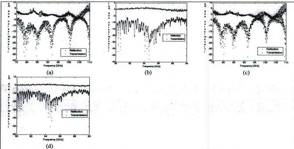
Figure 8. Magnitude of transmission and reflection response of (a) < 1 mg/mL NMPs mixed in Fluorinert at W-band, (b) same as (a) between 80-90 GHz, (c) 4 mg/mL of NMPs in Fluorinert at W-band, and (d) same as (c) between 80-90 GHz.
