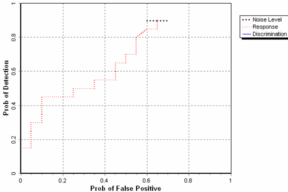
Figure 2. AN/PSS-14/handheld mine grid probability of detection for response and discrimination stages versus their respective probability of false positive over all ordnance categories combined.
