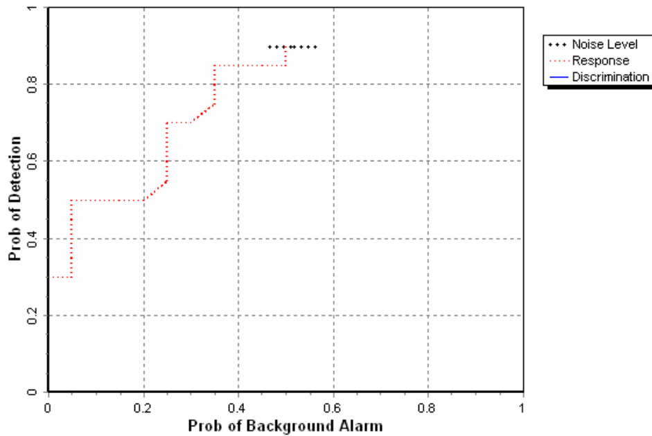
Figure 3. AN/PSS-14/handheld mine grid probability of detection for response and discrimination stages versus their respective probability of background alarm over all ordnance categories combined.
