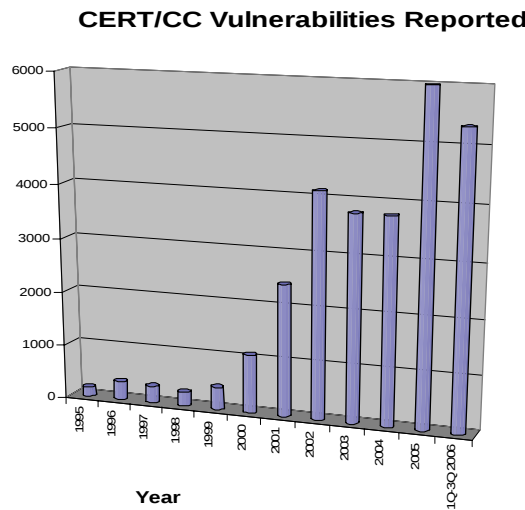
Figure 2: Vulnerability Reports 31
