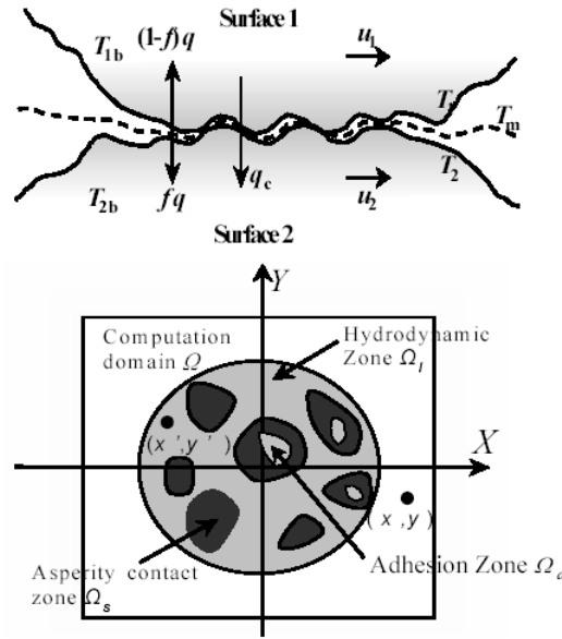
Figure 8 Physical model of thermal analysis for mixed lubrication in point contacts
