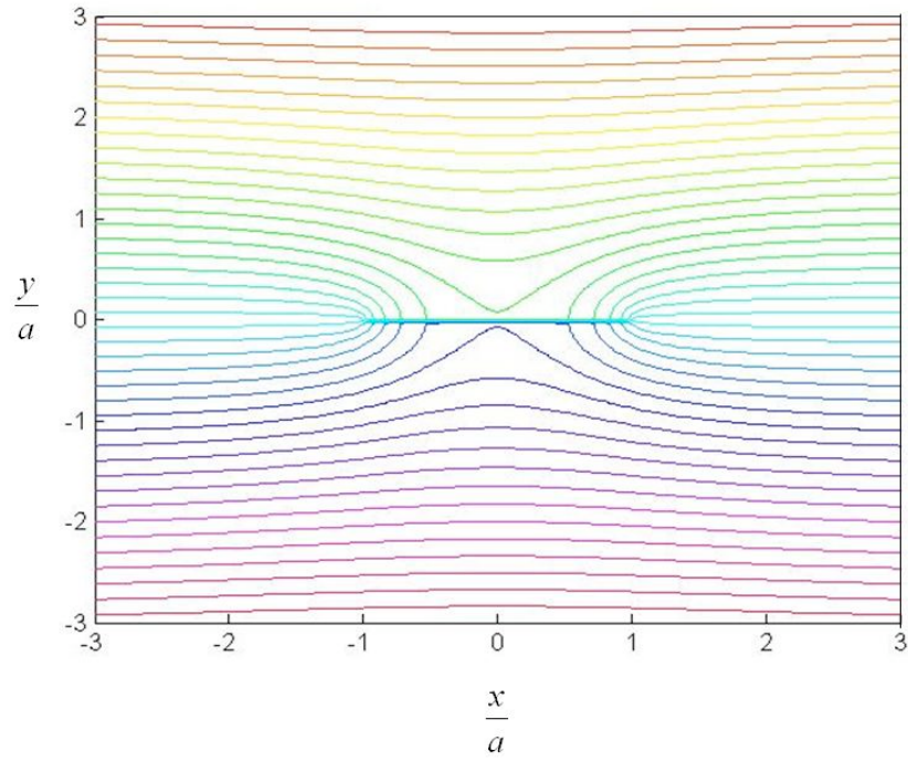
(a) The iso-valued contours of the total electric potential computed for the problem depicted by Fig. 4a
