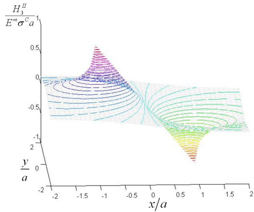
(b) The local magnetic field for the problem Fig. 4a
