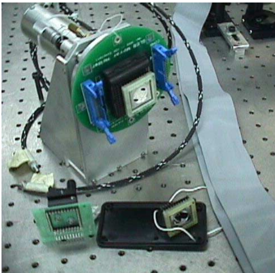
Figure 2. Photo and schematic of OKO deformable mirror used in described adaptive optics system. This unit has 37 active elements and measures 15 mm in diameter. Custom electronics drove the actuators.
