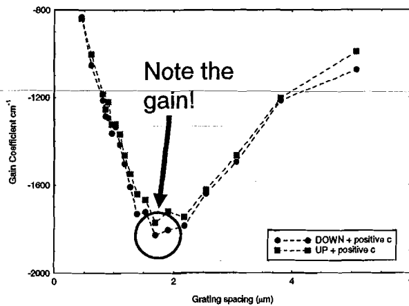
UP and DOWN + positive c twisted nematic TL205/0.01%Ce:SBN Hybrid Cell
