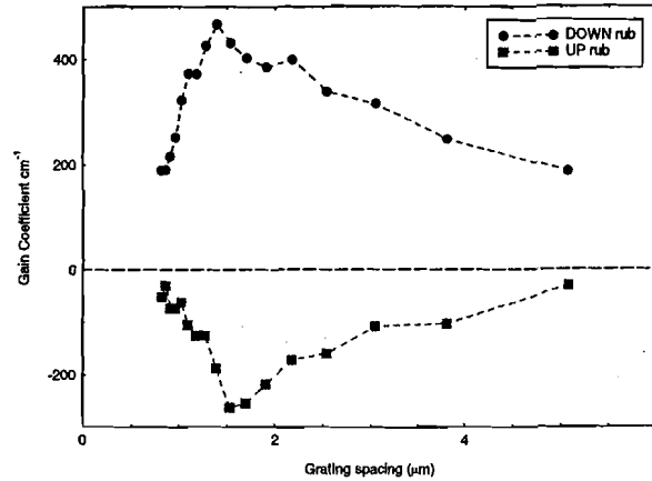
UP and DOWN + negative c twisted nematic TL205/0.01%Ce:SBN Hybrid Cell
