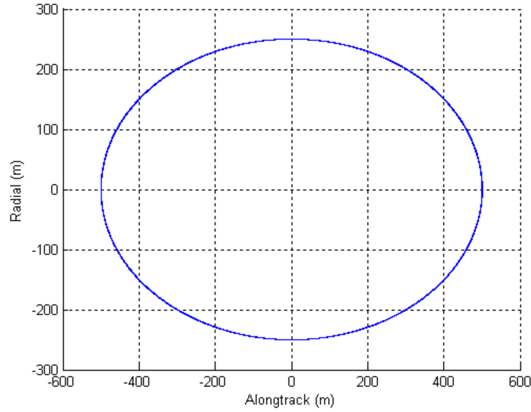
Figure 8: In-plane J_2 Invariant Relative Trajectory (100 Orbits)
