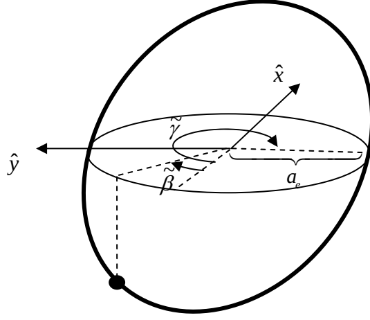
Figure 1: Relative Orbit
