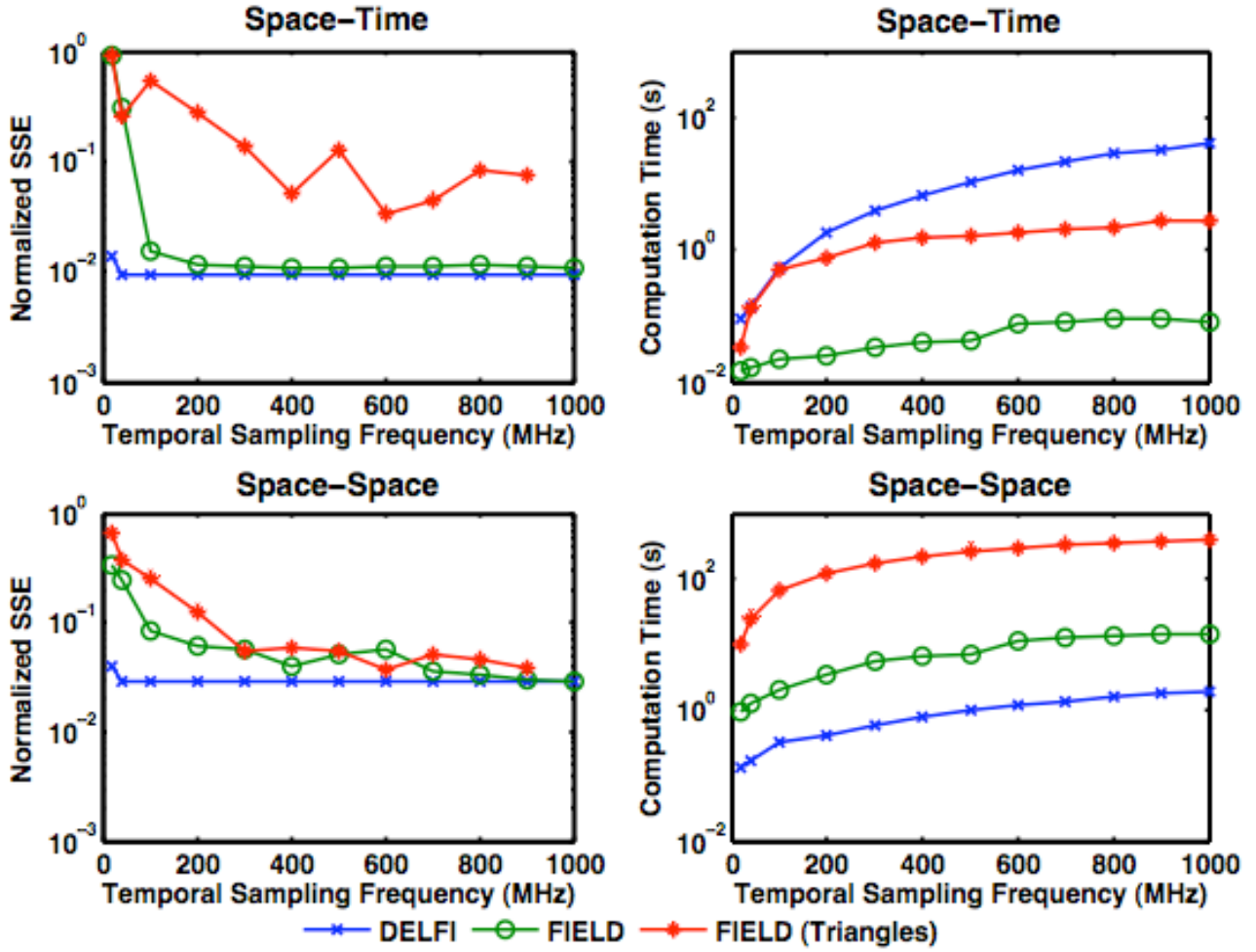
Figure 11: Simulation results comparing the speed and accuracy of DELFI and FIELD (both rectangular and triangular computational elements) for space-space and space-time responses. Note the high accuracy achieved for DELFI at even low sampling rates.
