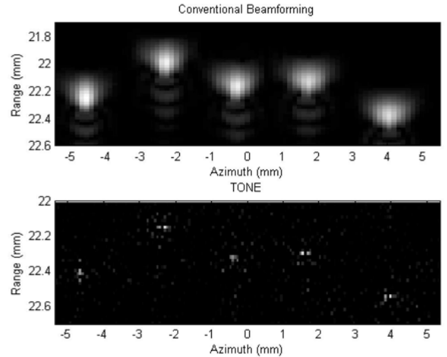
Figure 5. Conventional beamforming (top) and TONE beamforming (bottom) images of a set of 5 wires in water.
