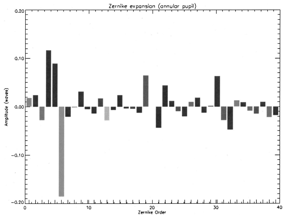
Fig. 5 Magnitude plot of the coefficients for the annular pupil Zernike polynomial modes.
