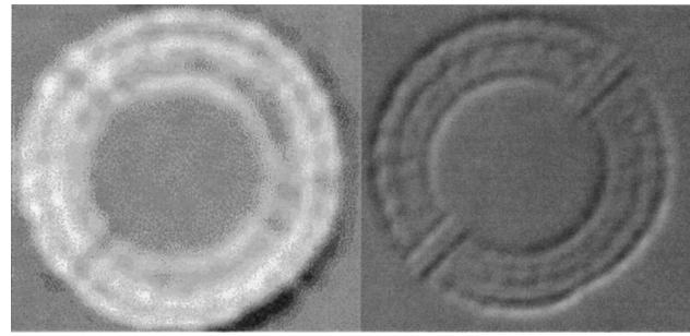
Fig. 2 Left: difference of the raw out-of-focus images of Fig. 1, an approximation of the \partial I/\partial z component of Eqs. (1) and (2); Right: phase map calculated from the left image using Eq. (2). Notice that there is an enhancement of the spiders in one direction while they are lost in the orthogonal direction.
