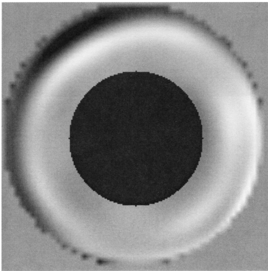
Fig. 7 Reconstruction of the wavefront using a 40-term expansion of the annular pupil Zernike fit of the data.
