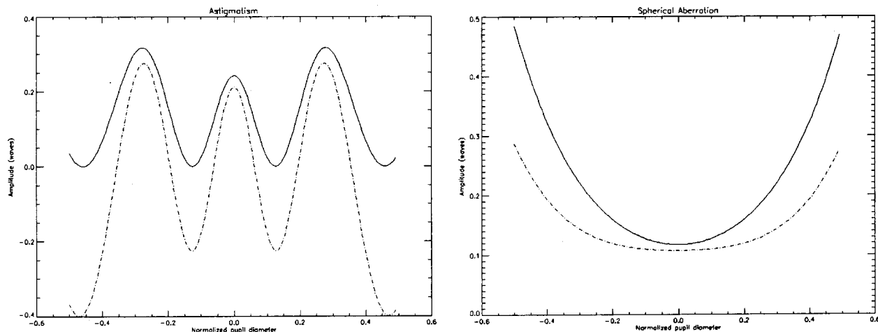
Fig. 6 Cross-cuts of the Zernike mode for astigmatism (left) and spherical aberration (right) for filled pupil (solid line) and annular pupil (dashed line).
