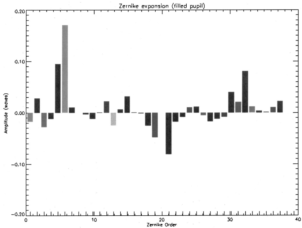
Fig. 4 Magnitude plot of the coefficients for the filled circular Zernike polynomial modes.
