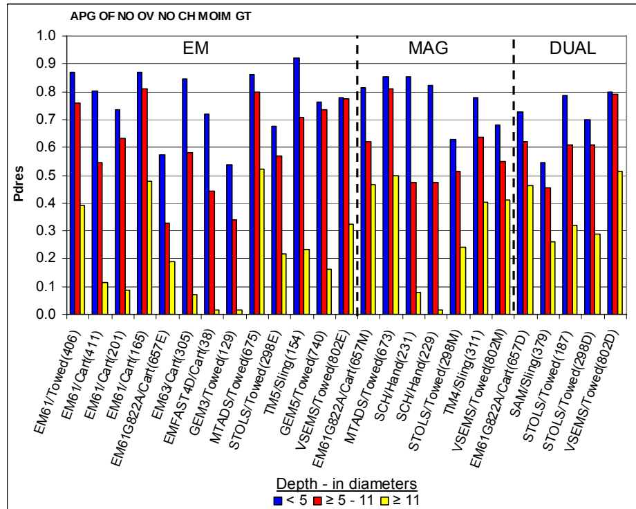
Figure 2.3.5-3b. P_d^{res} versus configurations for different depth ranges (< 5D, ≥ 5D to < 11D, ≥ 11D), APG open field, no challenge area, no overlaps.
