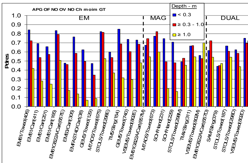
Figure 2.3.5-3a. P_d^{\text{res}} versus configurations for different depth ranges (< 0.3 m, ≥ 0.3 m to < 1 m, ≥ 1 m), APG open field, no challenge areas, no overlaps.
