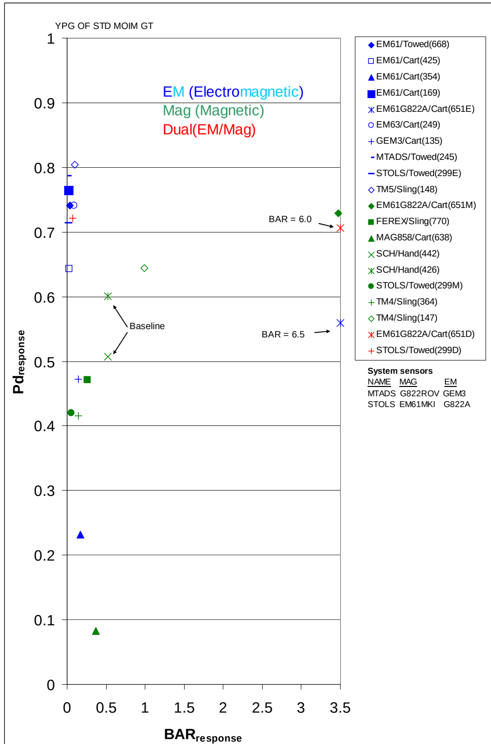
Figure 2.3.1-12. P_d^{\text{res}} versus \text{BAR}^{\text{res}} , YPG open field, Standard GT.
