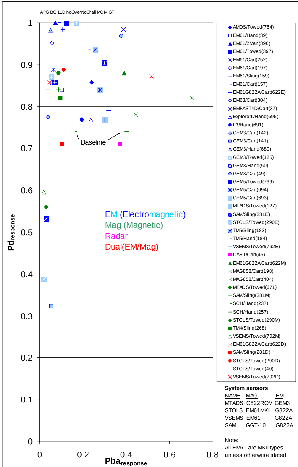
Figure 2.3.1-1. P_d^{\text{res}} versus P_{ba}^{\text{res}} , APG blind grid, 11D, No Overlap, No Challenge GT.
