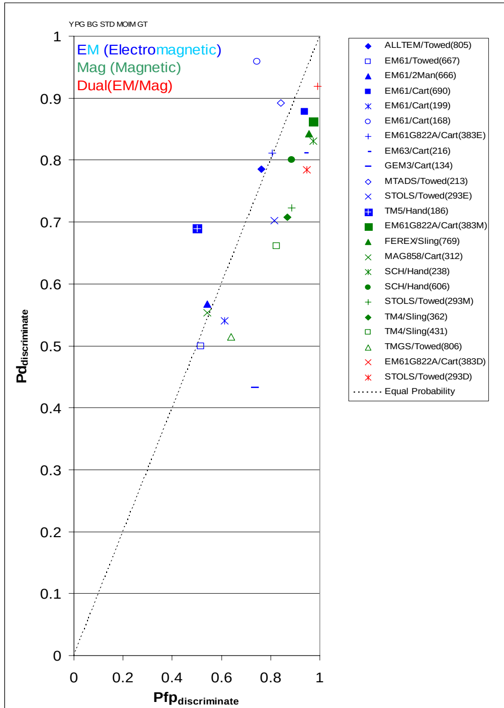
Figure 2.3.3-4. P_d^{\text{disc}} versus P_{fp}^{\text{disc}} , YPG blind grid.
