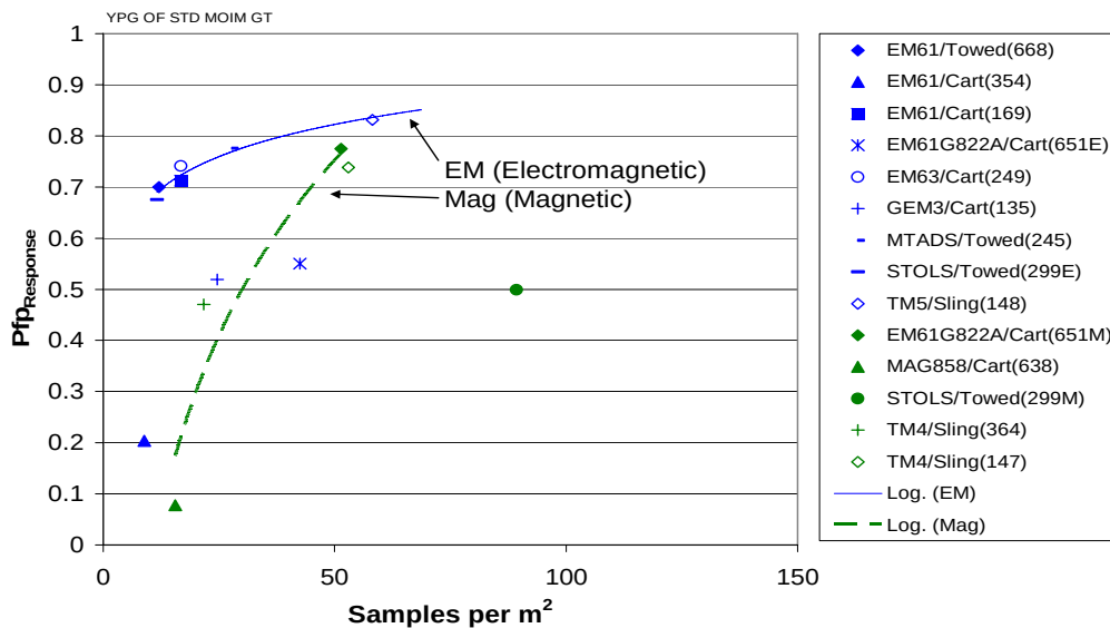
Figure 2.3.11-2. P_{fp}^{res} versus samples per m^2 , YPG open field.
