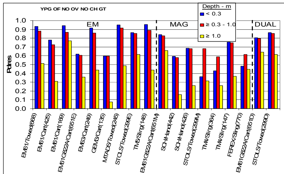
Figure 2.3.5-4a. P_d^{res} versus configurations for different depth ranges (< 0.3 m, ≥ 0.3 m to < 1 m, ≥ 1 m), YPG open field, no challenge area, no overlaps.
