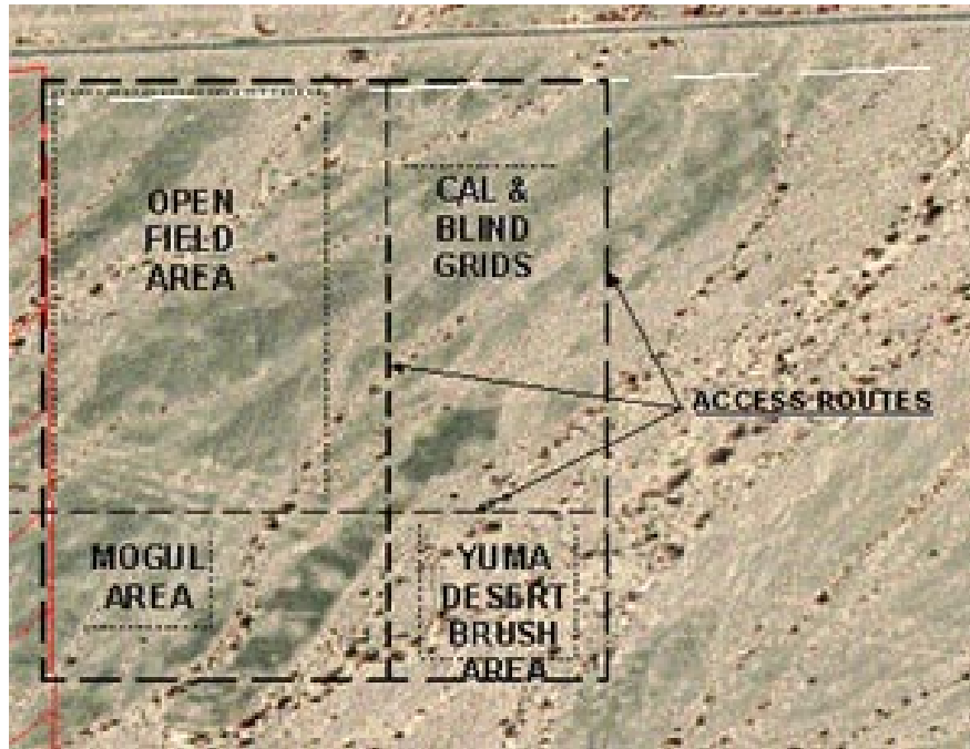
Figure 2.1-2. Layout of the YPG UXO test site.
