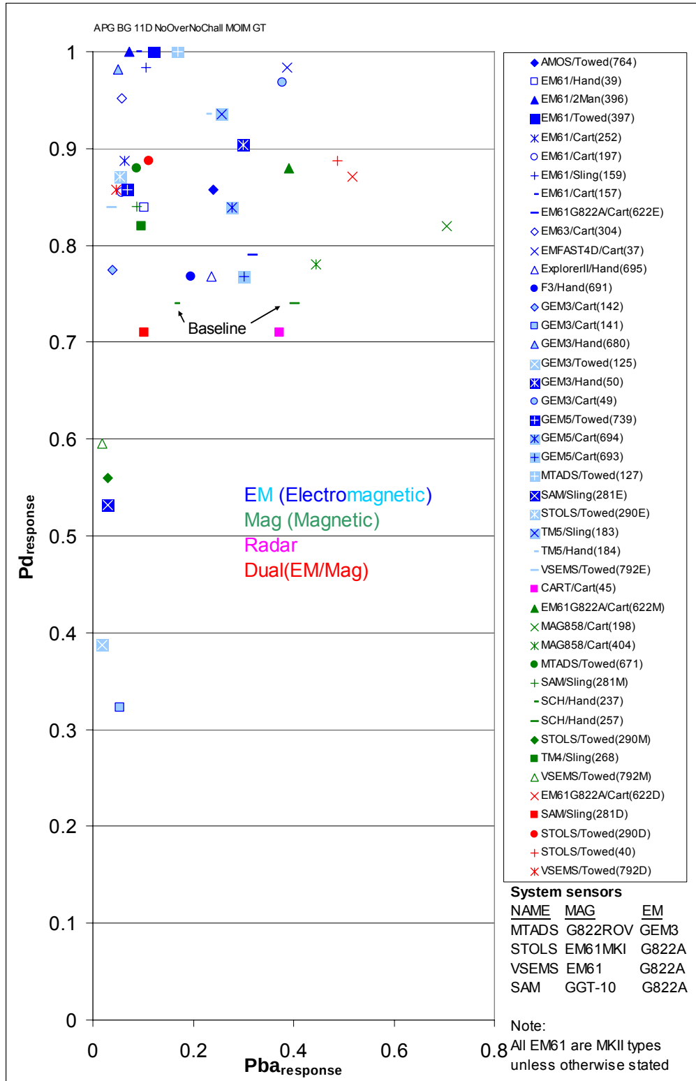
Figure 1. P_d^{\text{res}} , versus probability of background alarm ( P_{ba}^{\text{res}} ), APG blind grid results.
