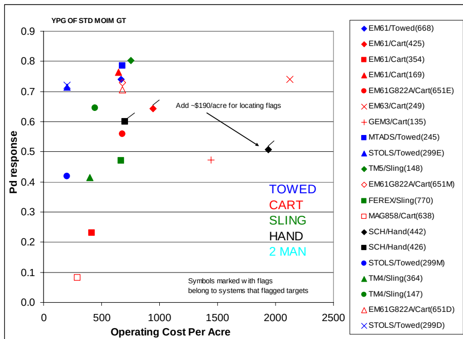
Figure 2.3.8-10. P_d^{\text{res}} , versus operating cost per acre, YPG open field.
