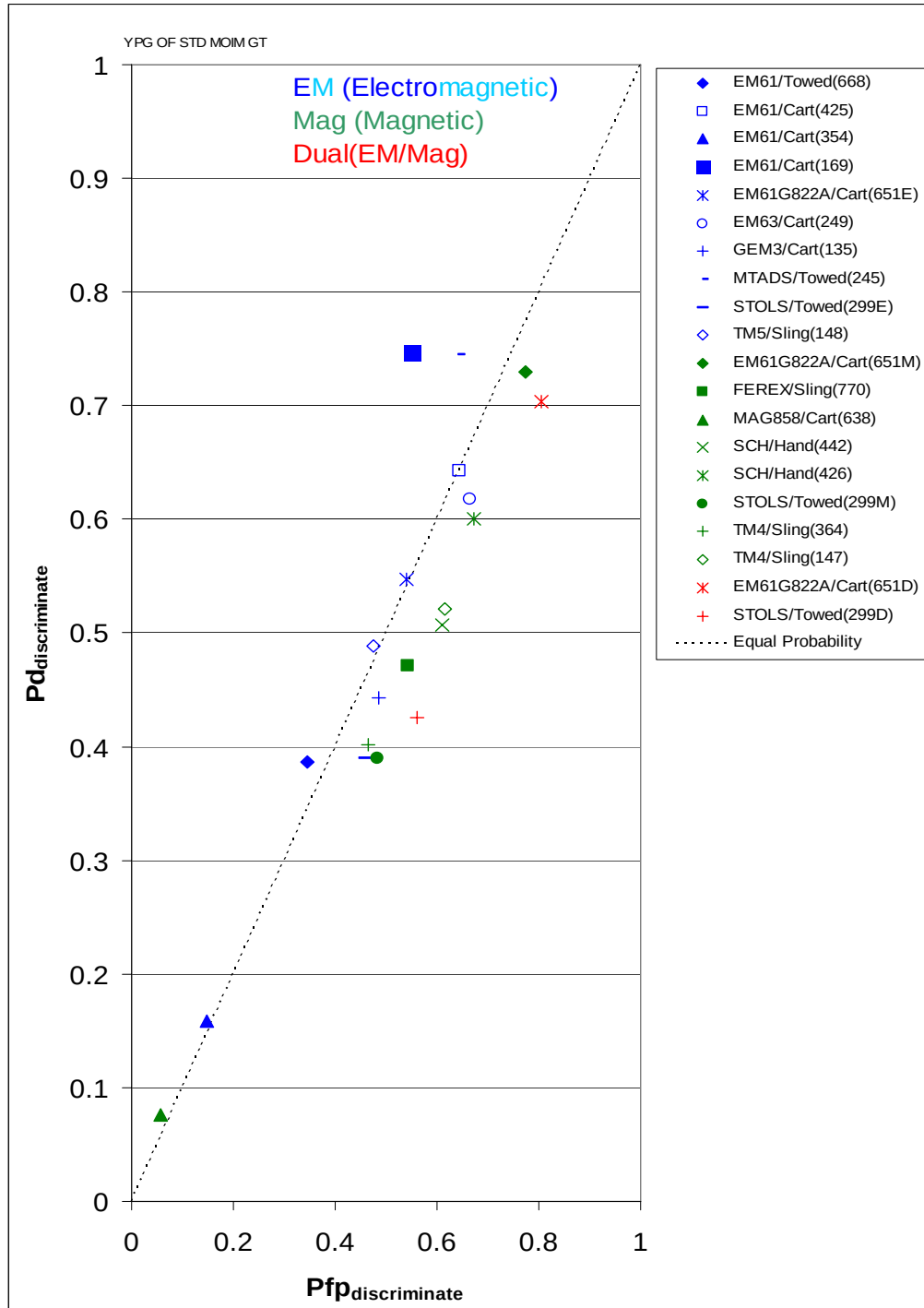
Figure 2.3.3-2. P_d^{disc} versus P_{fp}^{disc} , YPG open field.
