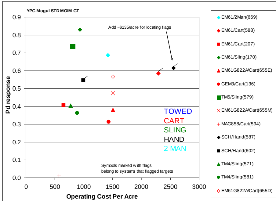
Figure 2.3.8-11. P_d^{\text{res}} , versus operating cost per acre, YPG moguls.
