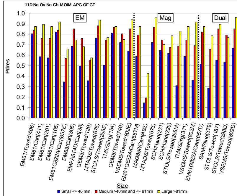
Figure 2.3.5-5. P_d^{\text{res}} versus demonstrator for size ranges, APG open field, 11D depth limit, no challenge area, no overlaps.
