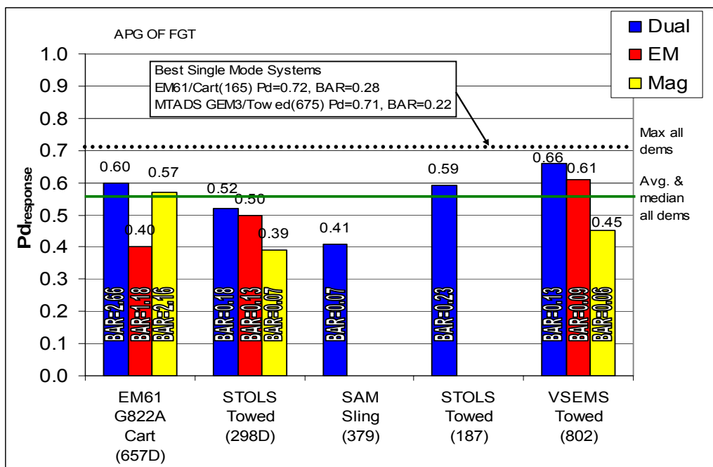
Figure 8. Dual system performance at APG open field, ferrous and non-ferrous items in GT.
