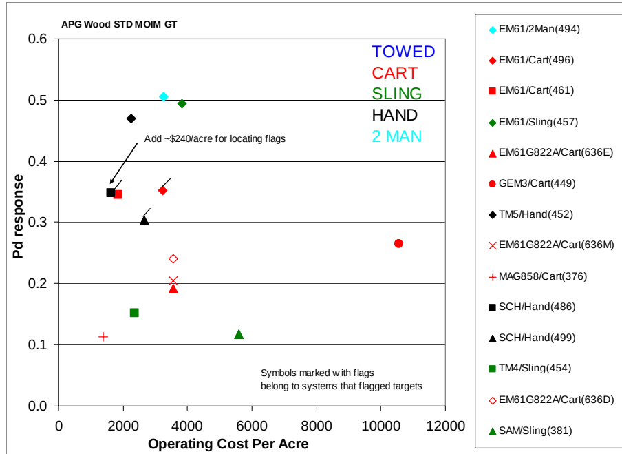
Figure 2.3.8-9. P_d^{\text{res}} , versus operating cost per acre, APG woods.
