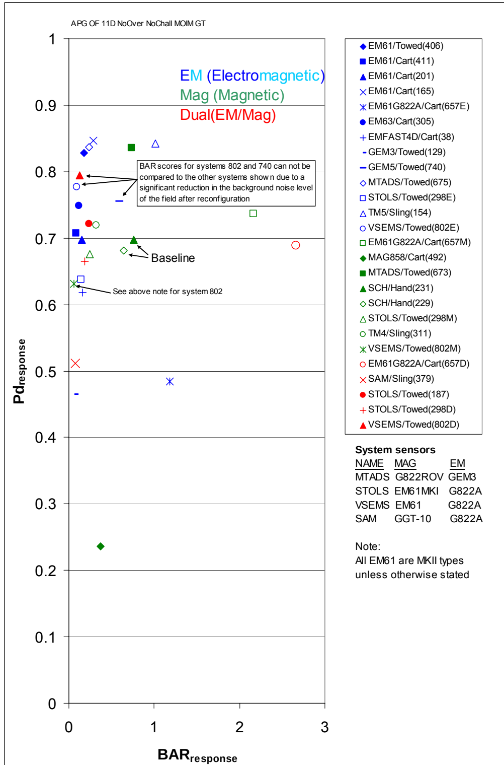
Figure 2. P_d^{\text{res}} versus \text{BAR}^{\text{res}} , APG open field results.
