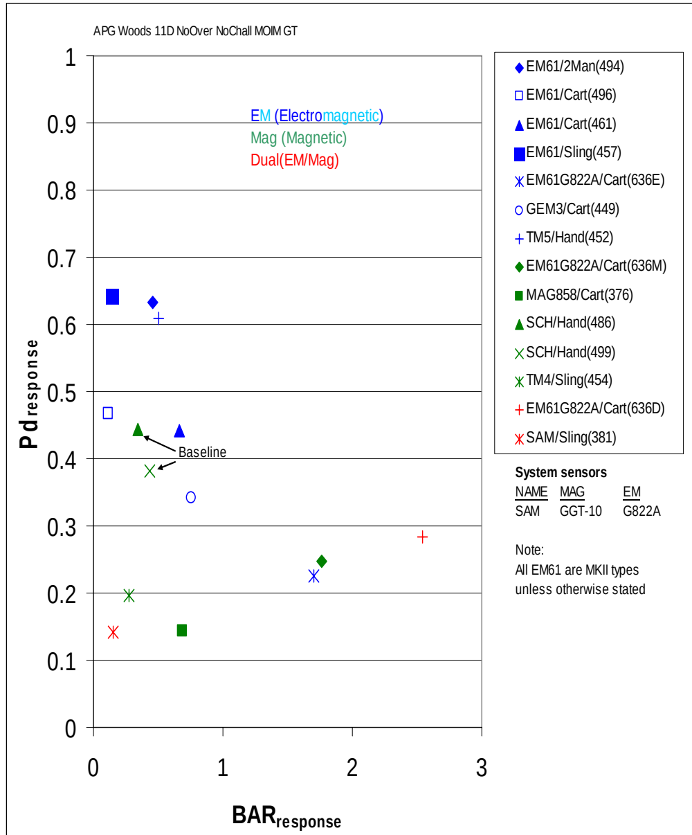
Figure 2.3.1-8. P_d^{\text{res}} versus \text{BAR}^{\text{res}} , APG woods, 11D, No Overlap, No Challenge GT.
