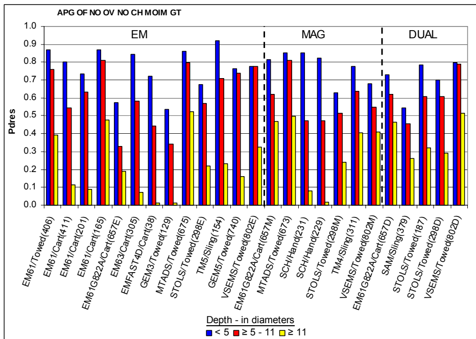
Figure 4. P_d^{\text{res}} as a function of depth in ordnance diameters, APG open field.
