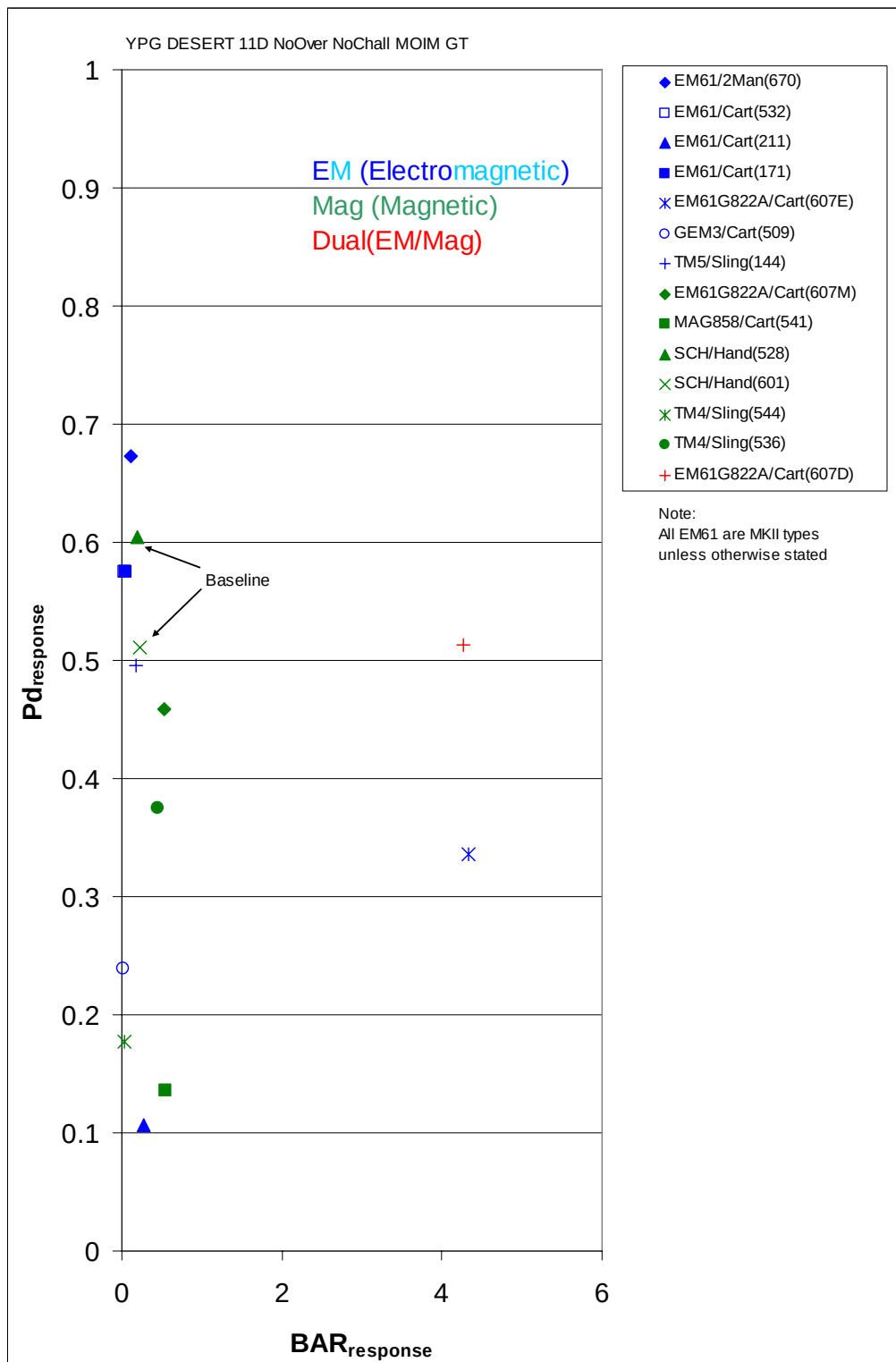
Figure 2.3.1-7. P_d^{\text{res}} versus \text{BAR}^{\text{res}} , YPG desert extreme, 11D, No Overlap, No Challenge GT.
