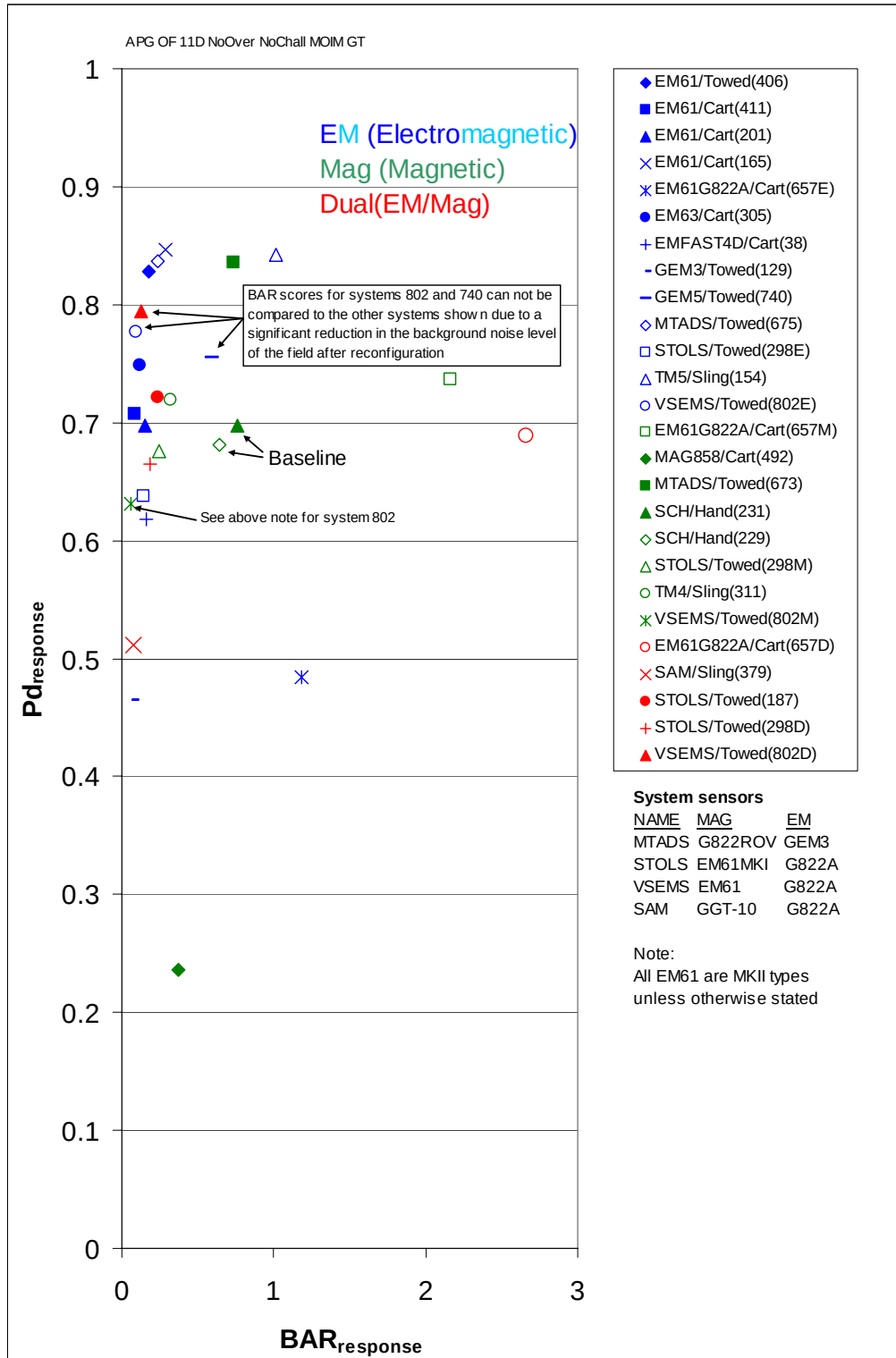
Figure 2.3.1-3. P_d^{\text{res}} versus \text{BAR}^{\text{res}} , APG open field, 11D, No Overlap, No Challenge GT.
