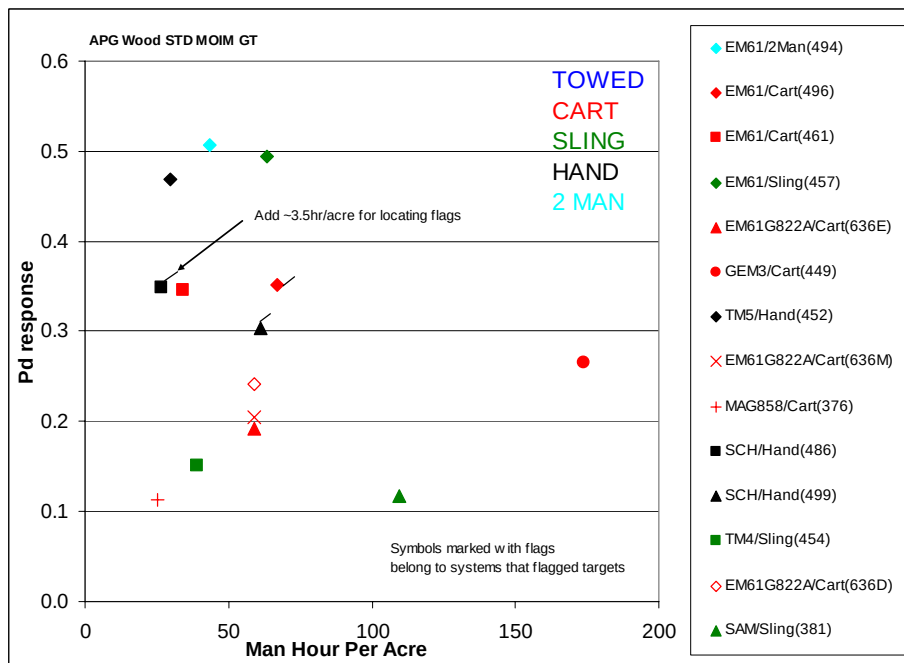
Figure 2.3.8-3. P_d^{\text{res}} , versus man-hours per acre, APG woods.
