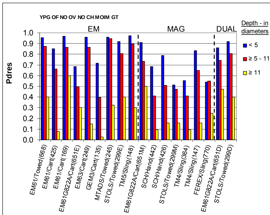
Figure 2.3.5-4b. P_d^{\text{res}} versus configurations for different depth ranges (< 5D, ≥ 5D to < 11D, ≥ 11D), YPG open field, no challenge area, no overlaps.
