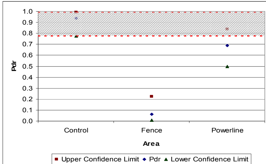
Figure 2.3.5-10. P_d^{\text{res}} for different challenge areas, with upper and lower confidence limits for VSEMS towed array, report No. 802D, APG.
