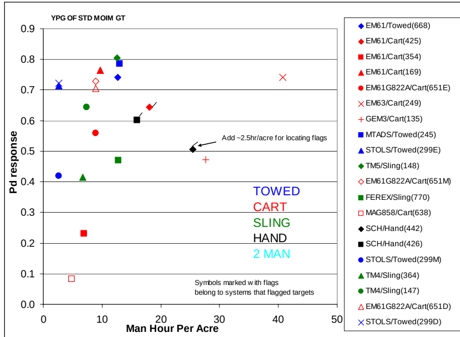
Figure 2.3.8-4. P_d^{\text{res}} , versus man-hours per acre, YPG open field.
