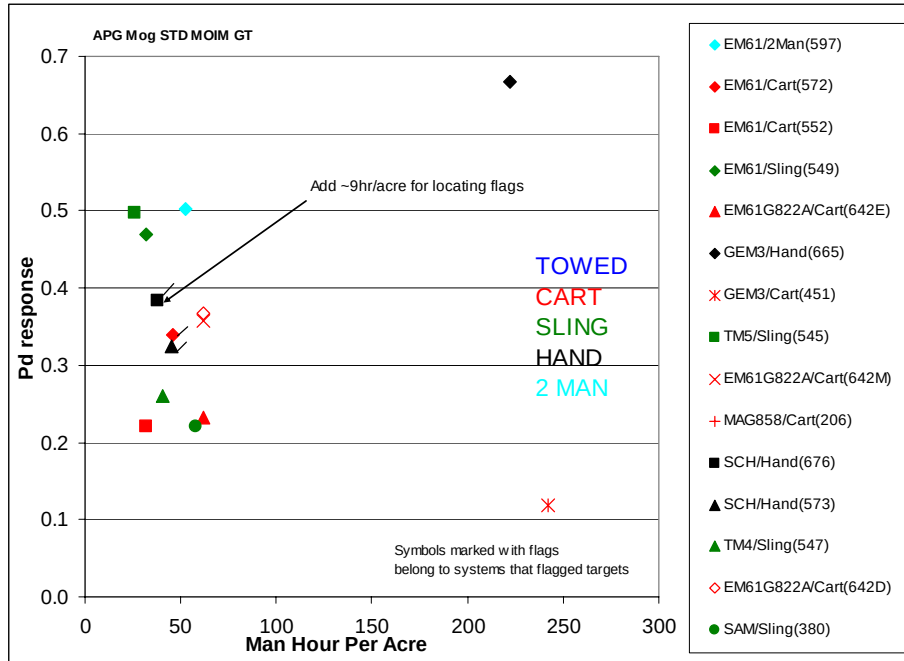
Figure 2.3.8-2. P_d^{\text{res}} , versus man-hours per acre, APG moguls.
