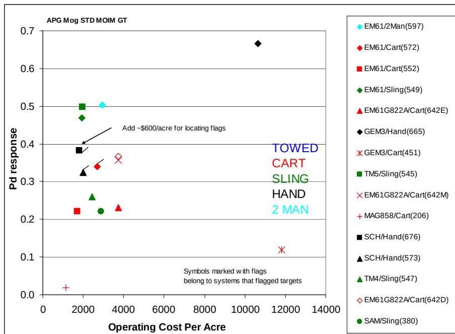
Figure 2.3.8-8. P_d^{\text{res}} , versus operating cost per acre, APG moguls.
