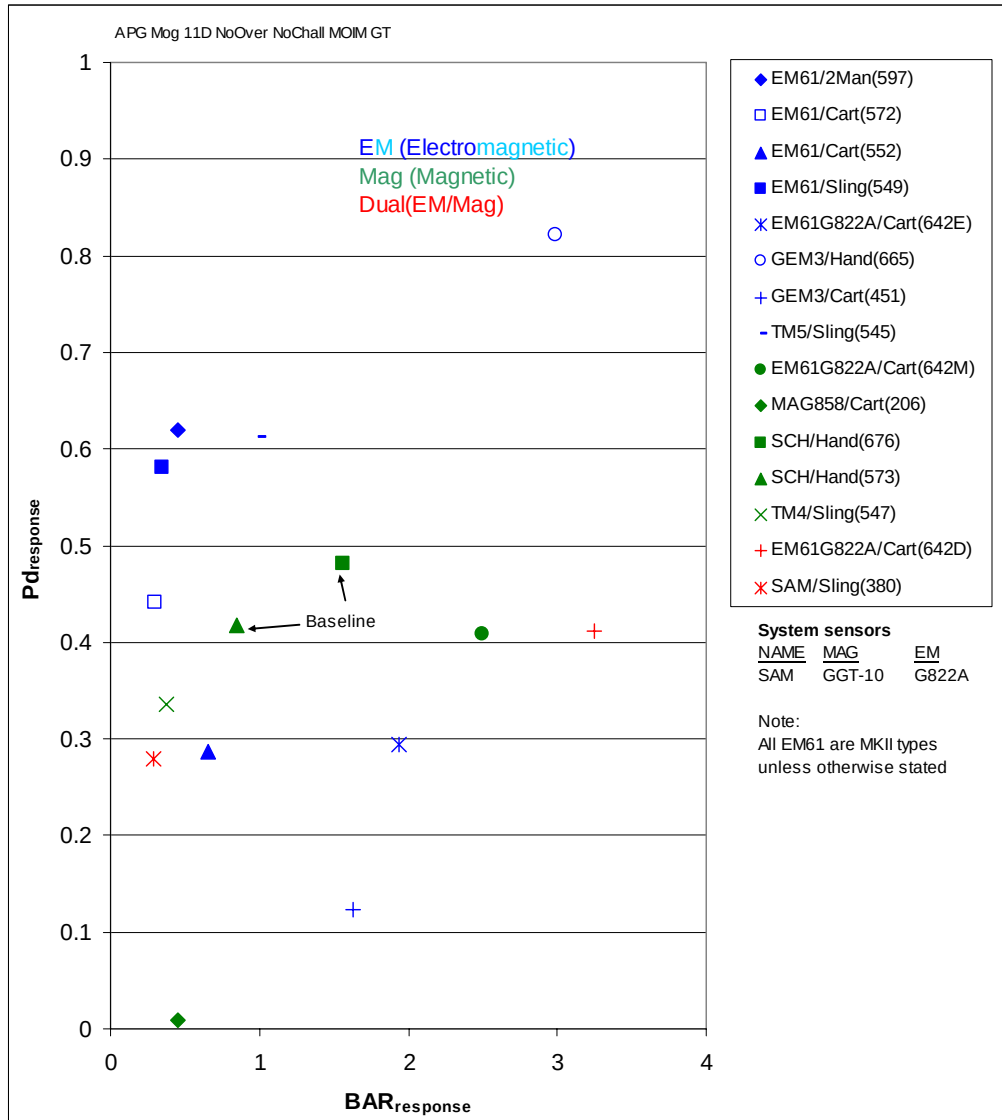
Figure 2.3.1-5. P_d^{\text{res}} versus \text{BAR}^{\text{res}} , APG moguls, 11D, No Overlap, No Challenge GT.
