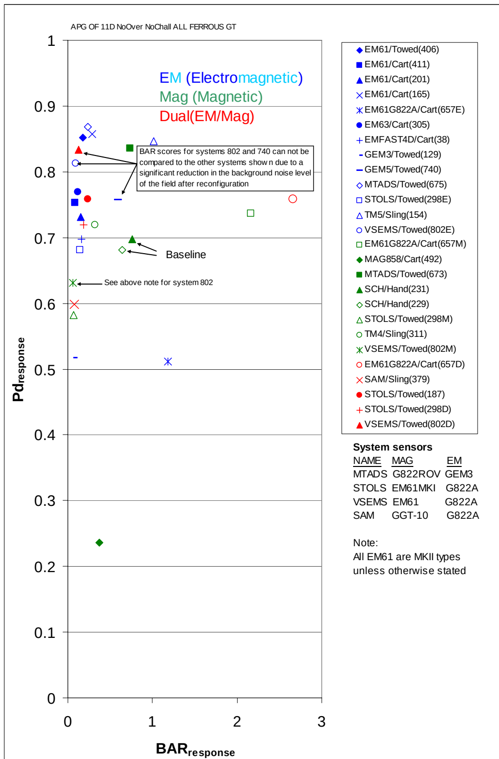
Figure 2.3.1-9. P_d^{\text{res}} versus \text{BAR}^{\text{res}} , APG open field, All ferrous, 11D, No Overlap, No Challenge GT.
