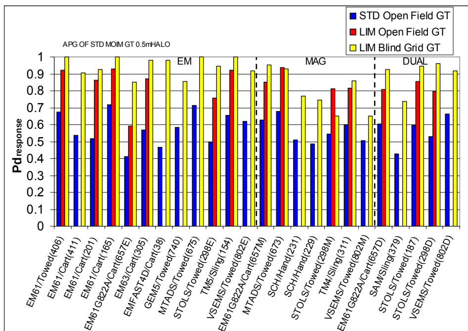
Figure 5. P_d^{\text{res}} for standard and LIM GT sets at APG.
