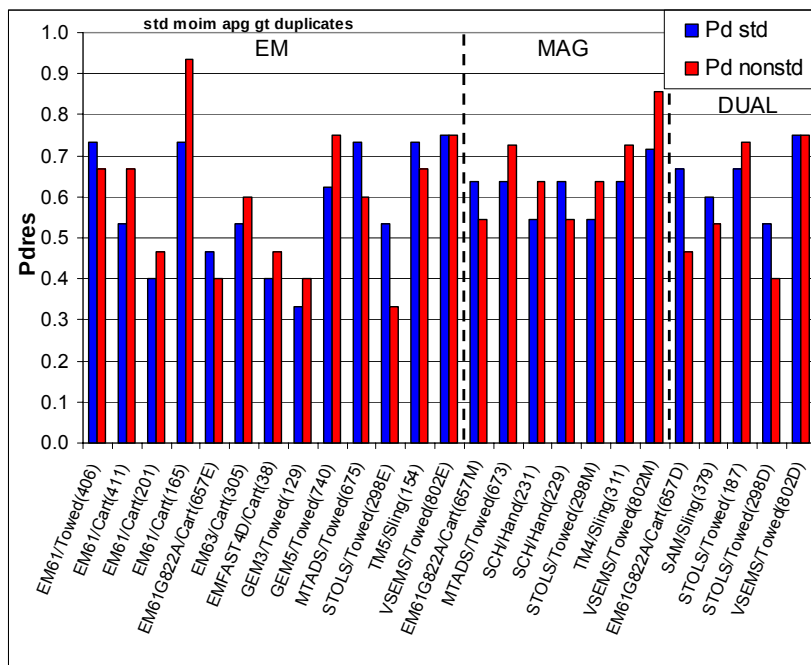
Figure 2.3.5-1. P_d^{\text{res}} versus demonstrator for standard and nonstandard GT, APG open field.
