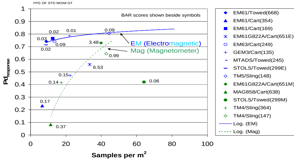
Figure 2.3.11-1. P_d^{res} versus samples per m^2 , BAR score labeled, YPG open field.
