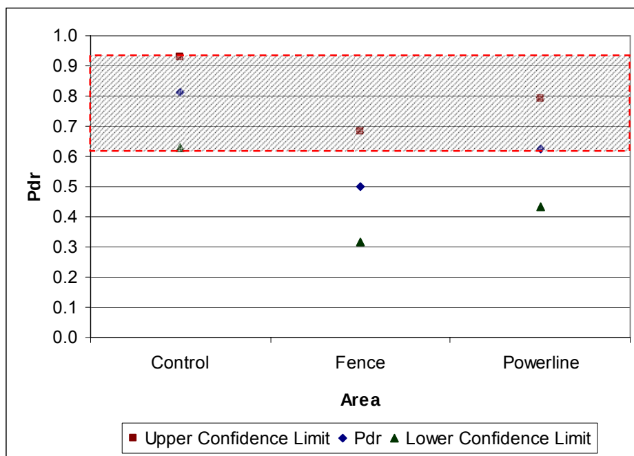
Figure 2.3.5-9. P_d^{\text{res}} for different challenge areas, with upper and lower confidence limits for GEM-5 towed array, report No. 740, APG.
