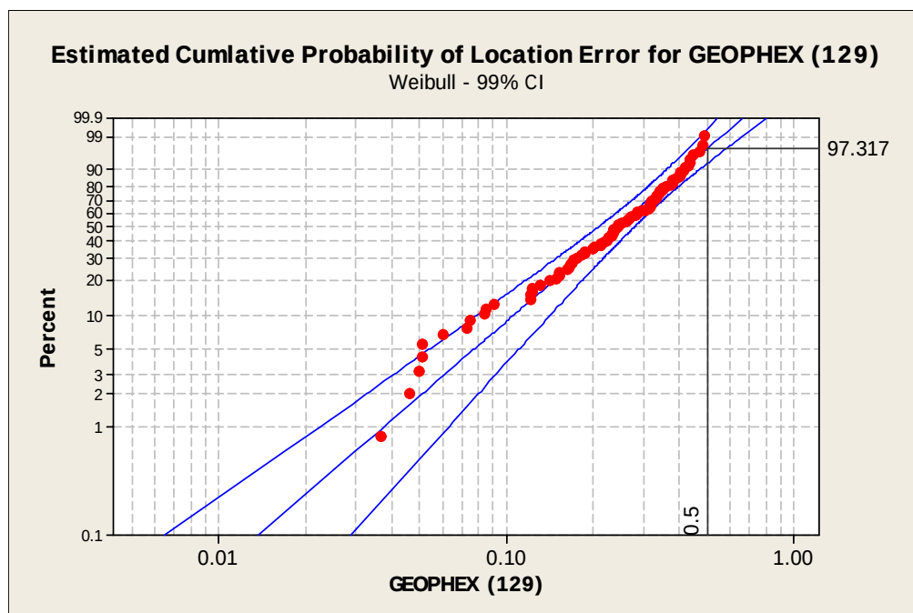
Figure F-2. Estimated Cumulative Probability of Location Error, Geopex, SR #129.
