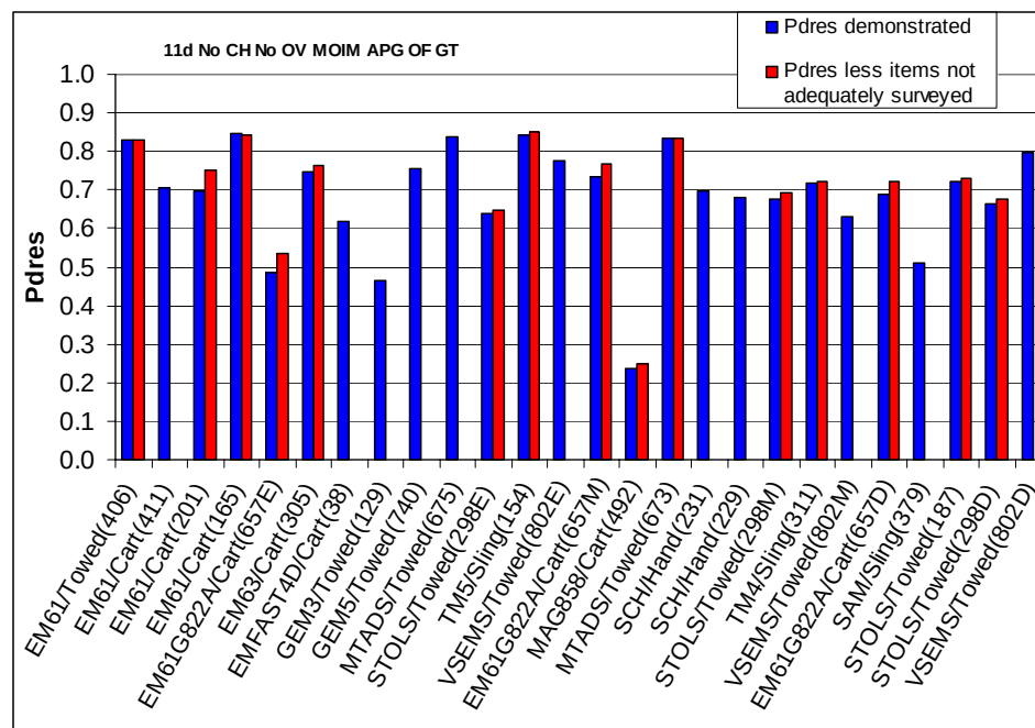
Figure 2.3.4-1a. P_d^{\text{res}} with and without items that were not adequately surveyed for each platform type, APG open field, 11D limit, no challenges, no overlaps.
