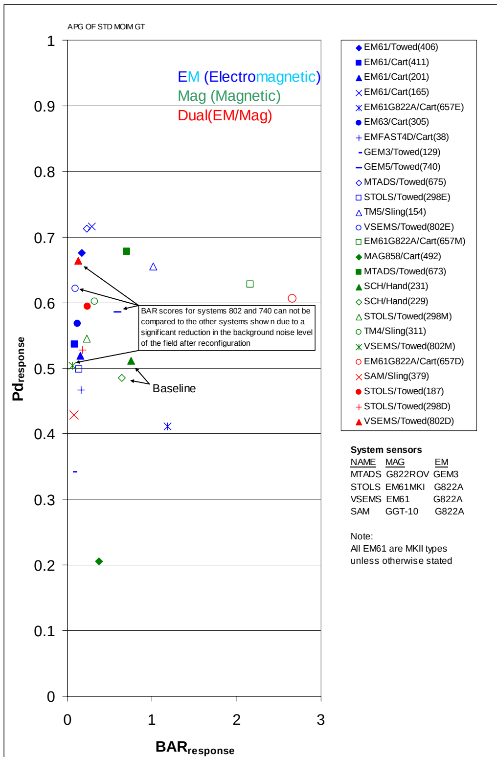
Figure 2.3.1-11. P_d^{\text{res}} versus \text{BAR}^{\text{res}} , APG open field, Standard GT.
