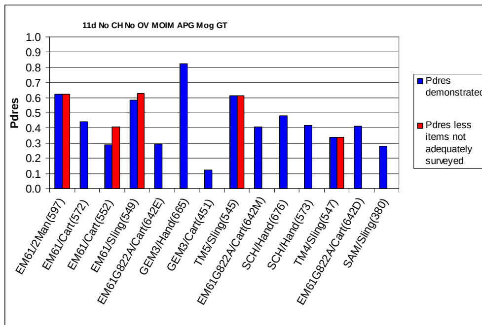
Figure 2.3.4-1c. P_d^{\text{res}} with and without items that were not adequately surveyed for each platform type, APG moguls, 11D limit, no challenges, no overlaps.
