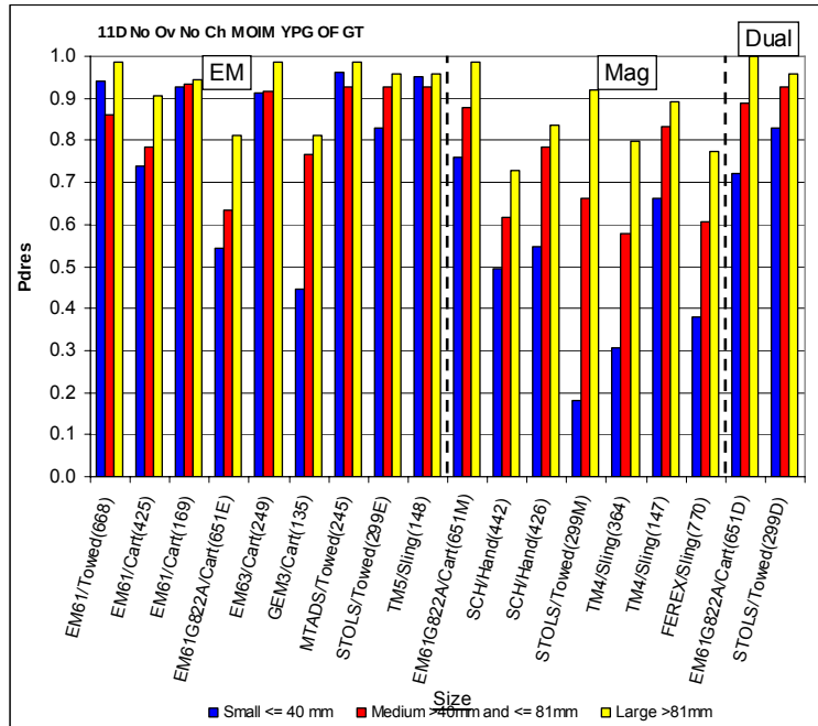
Figure 2.3.5-6. P_d^{\text{res}} versus demonstrator for size ranges, YPG open field, 11D depth limit, no challenge area, no overlaps.
