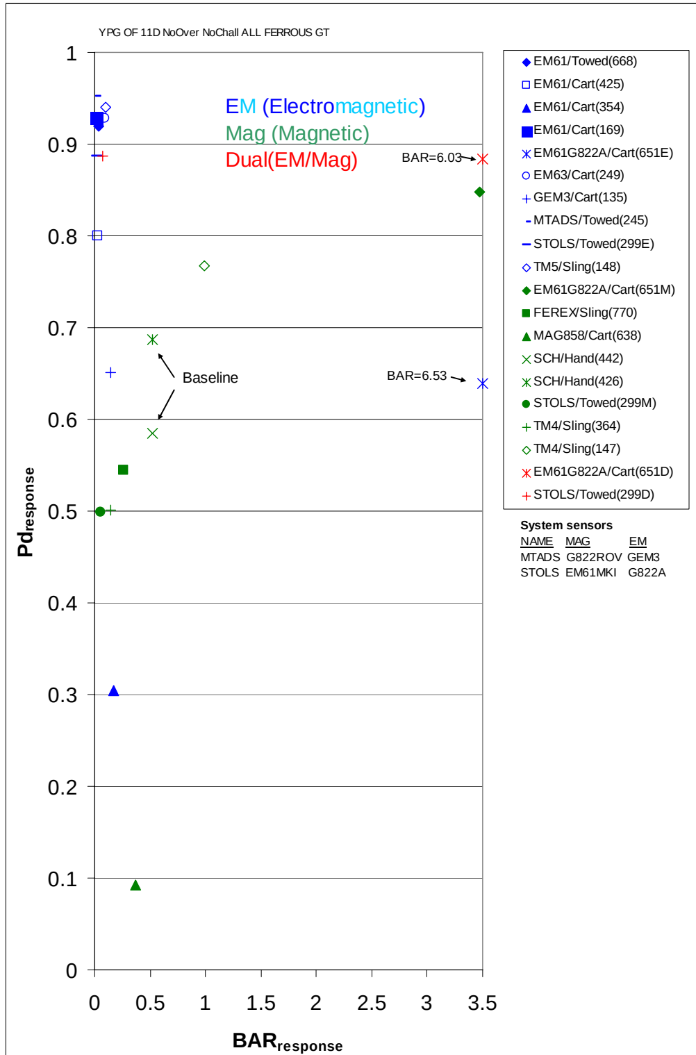
Figure 2.3.1-10. P_d^{\text{res}} versus \text{BAR}^{\text{res}} , YPG open field, All ferrous, 11D, No Overlap, No Challenge GT.
