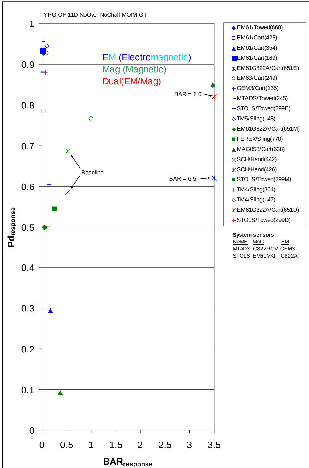
Figure 2.3.1-4. P_d^{\text{res}} versus \text{BAR}^{\text{res}} , YPG open field, 11D, No Overlap, No Challenge GT.
