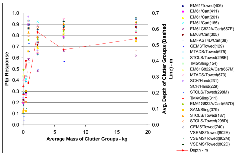
Figure 2.3.5-15a. P_{fp}^{res} , for different groups of clutter mass, APG open field, no challenge area, no overlaps.
