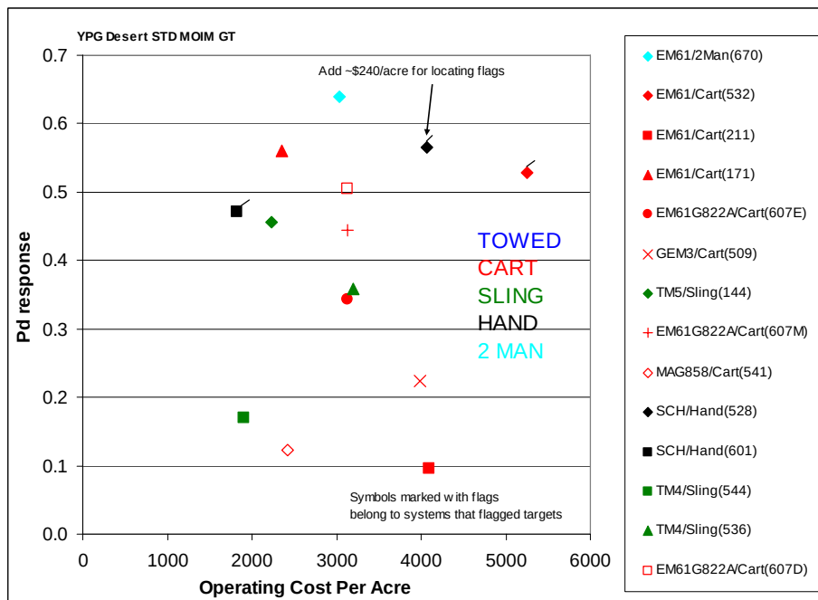
Figure 2.3.8-12. P_d^{\text{res}} , versus operating cost per acre, YPG desert extreme.
