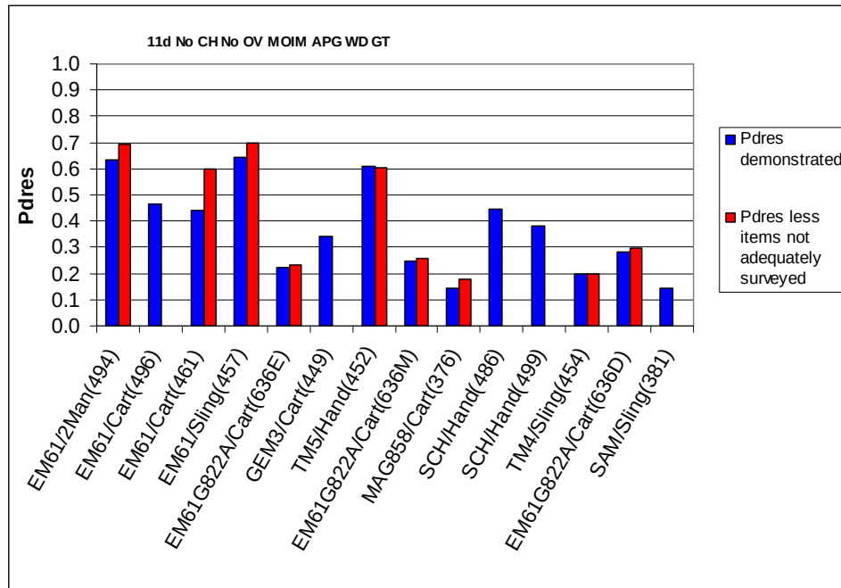
Figure 2.3.4-1b. P_d^{\text{res}} with and without items that were not adequately surveyed for each platform type, APG woods, 11D limit, no challenges, no overlaps.
