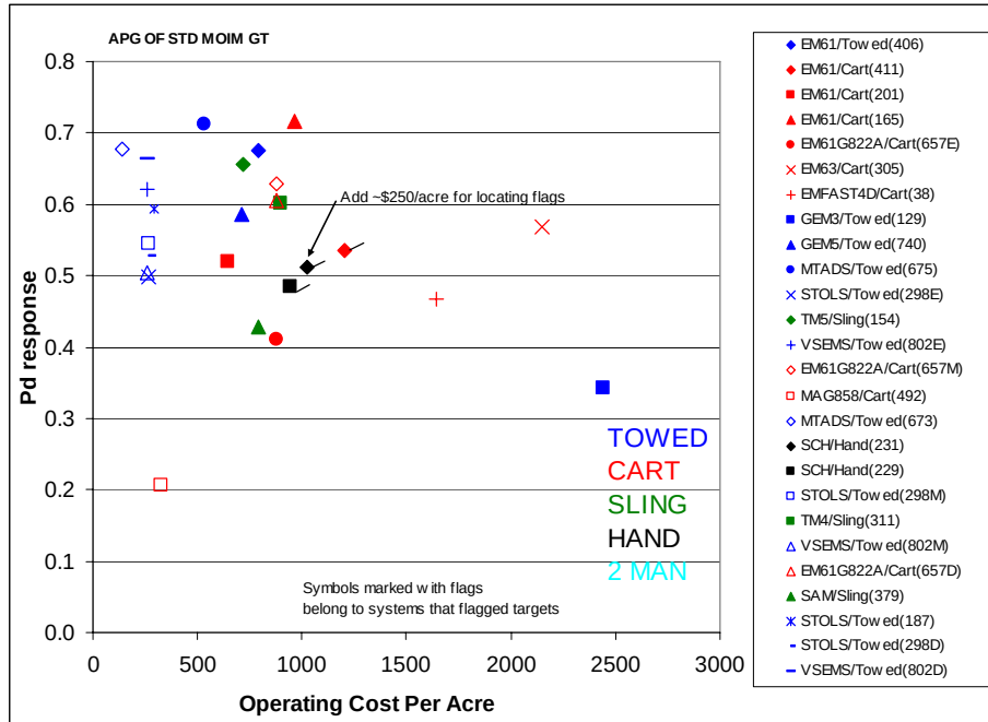
Figure 2.3.8-7. P_d^{\text{res}} , versus operating cost per acre, APG open field.
