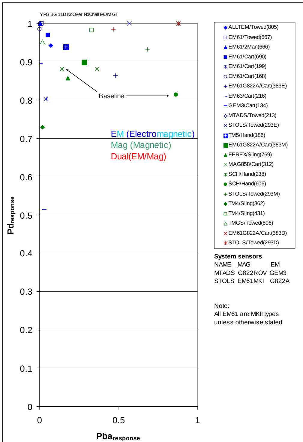
Figure 2.3.1-2. P_d^{\text{res}} versus P_{ba}^{\text{res}} , YPG blind grid, 11D, No Overlap, No Challenge GT.
