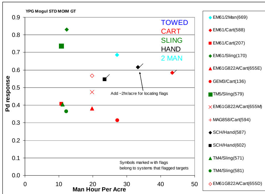
Figure 2.3.8-5. P_d^{\text{res}} , versus man-hours per acre, YPG moguls.
