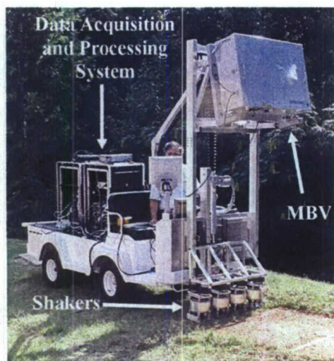
Figure 3. Functional prototype of a confirmation sensor with mechanical shakers and multiple-beam vibrometer.
