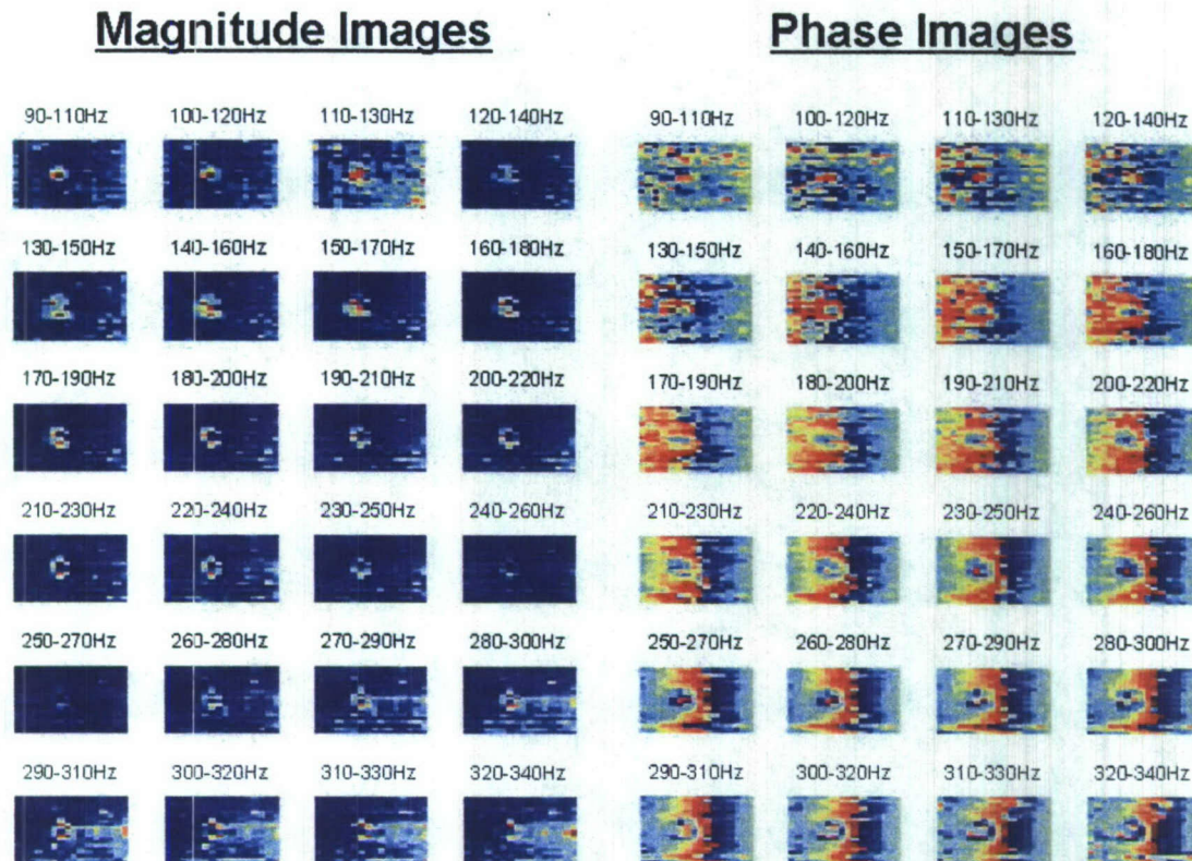
Figure 16. Magnitude and phase velocity images of a EM12 antitank landmine simulant.
