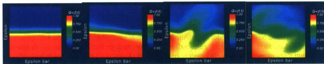
Figure 5. Distribution function of electrons in a strong electric field as a function of time, starting on the left before the field is turned on, and increasing in units of time equal to about one third of the Bloch period for each time step. Note how the distribution of electrons gets mixed with a swirling motion as the time increases, and how the occupation of states becomes more evened out as time increases.
