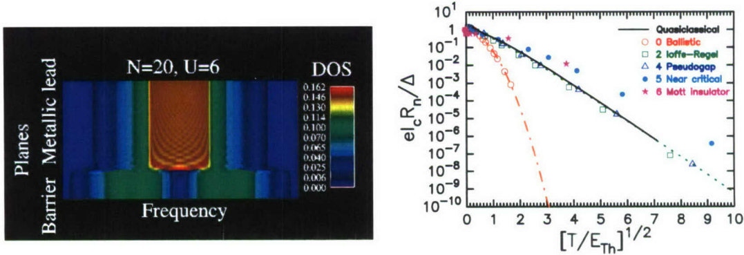
Figure 2. The left panel shows the many-body DOS of an N=20 thick barrier embedded in a metallic-lead sandwich (only half of the junction is shown). Note the Friedel oscillations in the metal, and the mismatch of the bands due to the insulating behavior in the barrier. The right panel shows a plot of the JJ figure of merit divided by the superconducting gap, versus the square root of the ratio of the temperature to the Thouless energy. This formulation provides a clear distinction between the ballistic case (lowest curve), the diffusive case (middle curves with the quasiclassical approach in the solid black line) and the correlated insulator case (uppermost curves).
