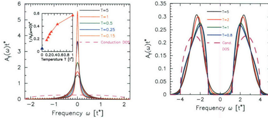
Figure 3. F -electron DOS for the FK model on a Bethe lattice with U=1 (left) and U=5 (right). The conduction electron DOS is given by the dashed magenta curve. Note the sharp peak in the left panel, and the gap opening in the right. The curves are for different temperatures. These results were checked against a number of different moment sum rules and spectral formulas, and our error estimates are on the order of a few percent (pointwise). Inset in the left panel is a plot of the inverse DOS at zero frequency versus temperature, indicating a peak height of about 20 at T=0 . We cannot rule out a divergence of the peak though, which has been verified by numerical renormalization group calculation.
