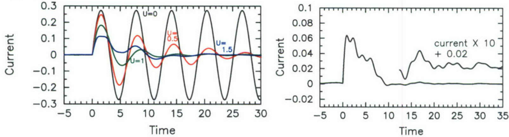
Figure 4. Decay of the Bloch oscillations as a function of time for different metallic systems (left) and for a small-gap Mott insulator (right). Note how the increase of scattering quenches the oscillations more rapidly, but that the calculations have not yet reached the steady state. In the insulator, the current has a much more irregular behavior that is difficult to describe via any form of regular oscillations.
