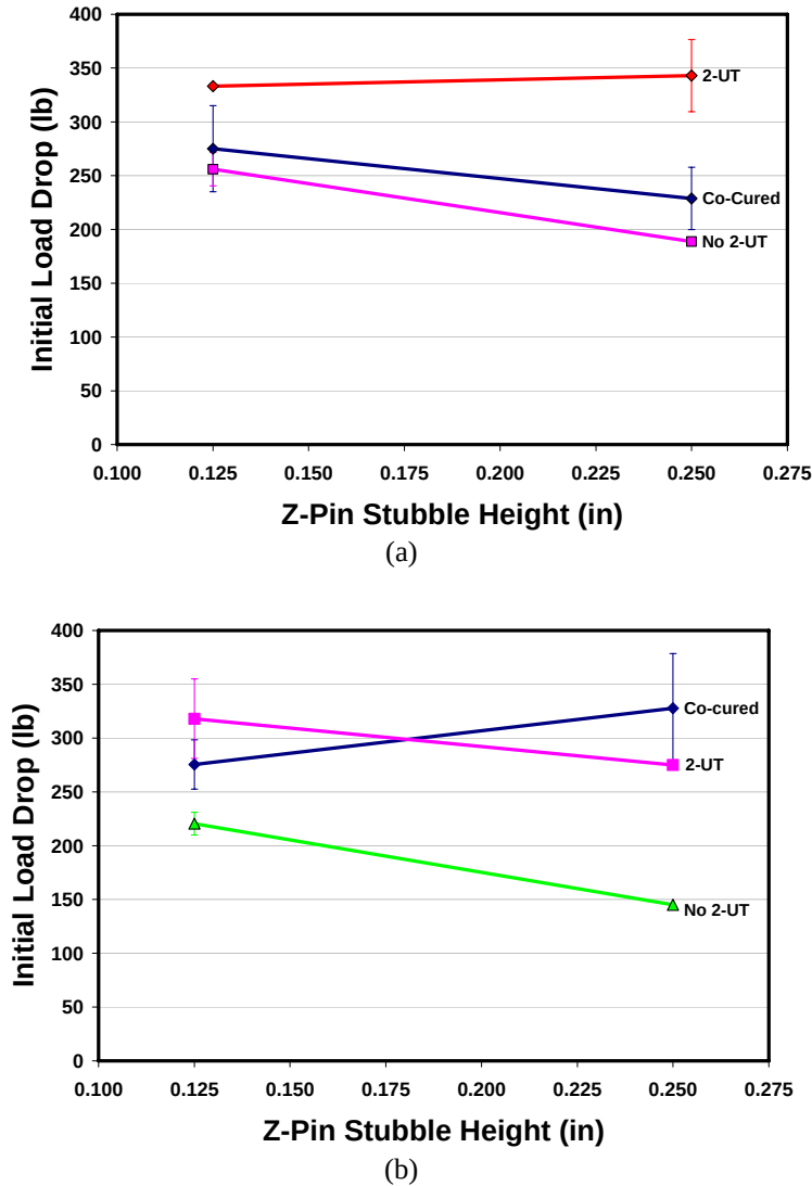
Figure 10: Effect of 2 nd Ultrasonic Step on Initial Mode I Load Drop at (a) 2% and (b) 4% Aerial Density
