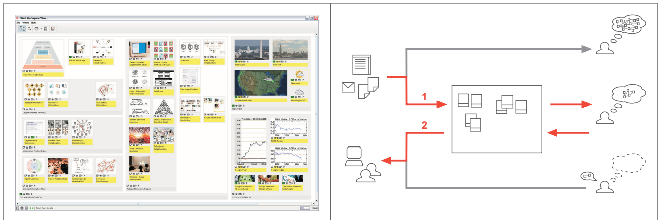
Figure 2: Workspace View
