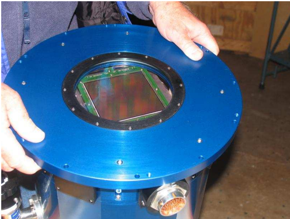
Figure 4: Dewar of 10k camera with STA1600 chip. This monolithic CCD detector has 10,560 by 10,560 light sensitive pixels of 9\mu\text{m} size. First light was obtained 2007 Oct 09 at the USNO astrograph. The URAT focal plane assembly will accommodate 4 of these detectors.
