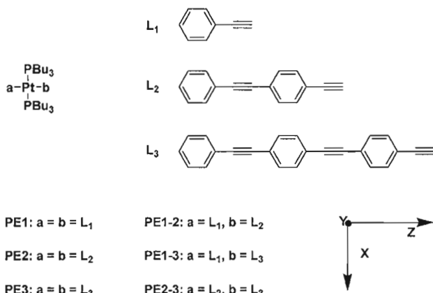
Figure 1. Chemical formulas and nomenclature. Arrows show molecular axes. Nomenclature for the asymmetric compound a -Pt( PBu_3 ) _2 - b , designated as PEa-b , labels two ligands of the compound. In discussions below, ligand a is designated as the “left ligand” and ligand b is the “right ligand”. When a = Cl , the chromophore is designated as “ half-PEb ”. The butadiyne PE_n-C\equiv C-C\equiv C-PE_n is labeled as “ PE n -BD ”.
