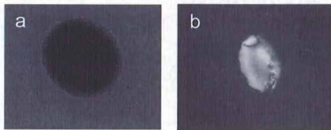
FIGURE 6 (a) Formation of micro-domain structure immediately after switching off the He-Ne laser beam. (b) Direct observation of critical opalescence when scanning the red laser beam across the sample.
