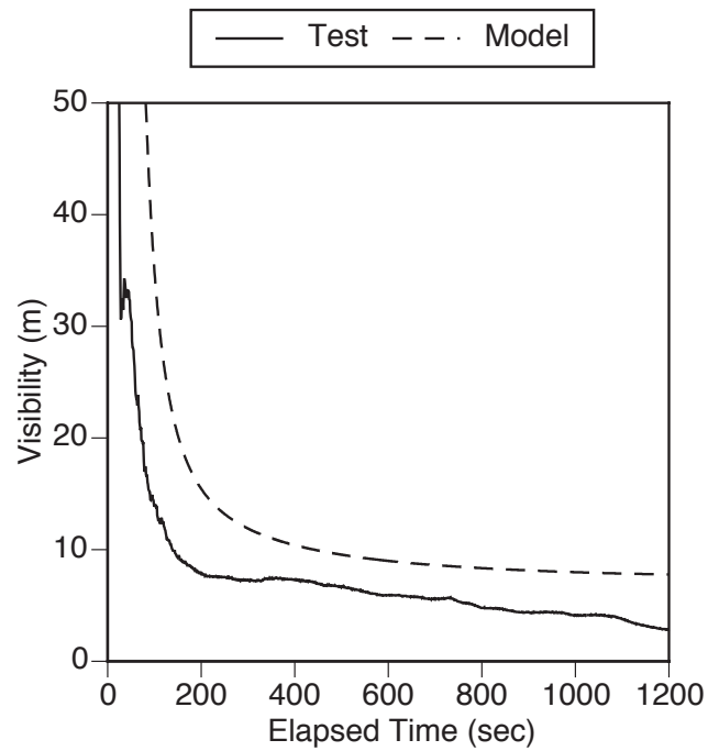
Figure C-7. Control Room Visibility
