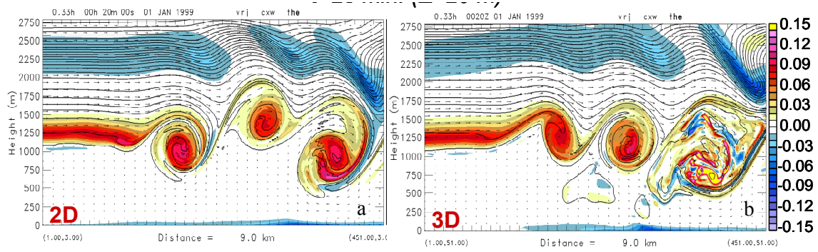
Figure 1. Vertical cross section of wind vectors, potential temperature (K) and y-component of the horizontal vorticity ( \text{s}^{-1} ) (color scale shown at right) for (a) two-dimensional simulation of sub-rotors and (b) three-dimensional simulation after 20 min. The horizontal and vertical grid increments are 20 m. Tick marks along the abscissa are shown every 250 m.
