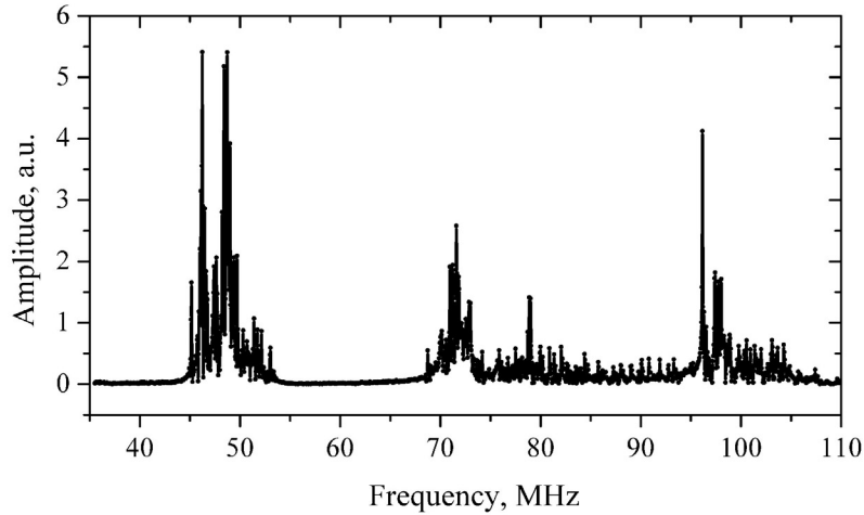
Figure 2. Frequency response of 20 \times 20 paddle array with 2\text{-}\mu\text{m} -long connecting arm. Data acquired by driving a paddle at the center of the array and detecting the vibrations at the next paddle.
