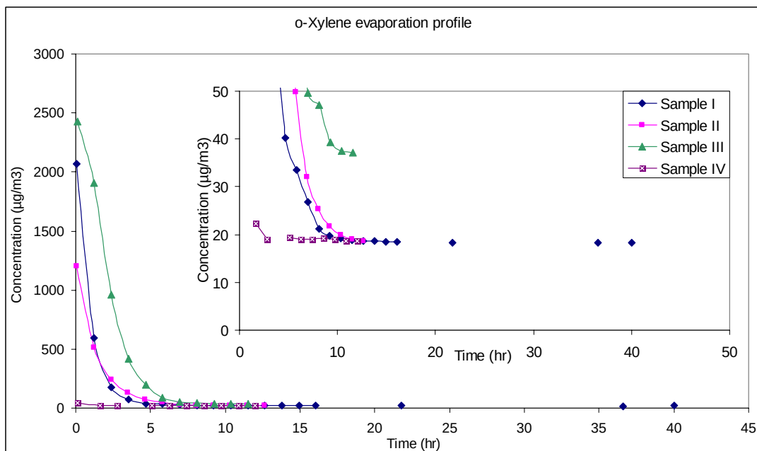
Figure 37. Concentration-time courses of o-xylene in the vapor phase during evaporation of JP-8 samples I to IV at -10\text{ }^{\circ}\text{C} . The discontinuities in the measurements are due to the detection limit of the analytical configuration of \text{ca } 18\text{ }\mu\text{g}/\text{m}^3 .
