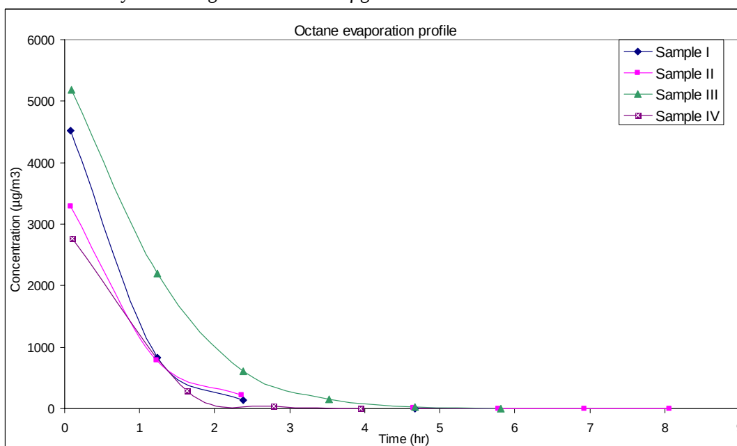
Figure 32. Concentration-time courses of octane in the vapor phase during evaporation of JP-8 samples I to IV at -10^{\circ}\text{C} . Within 8-9 h the vapor concentration has dropped below the detection limit of the analytical configuration of \text{ca } 0.5\text{-}2 \mu\text{g}/\text{m}^3 .
