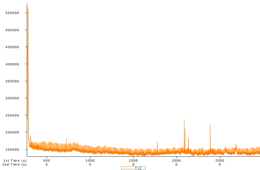
Figure 20. The modulated chromatogram (TIC) of the vapor at 80 hr after start of the evaporation of the jet fuel sample I, the KC135 JP-8, at -10 °C.
