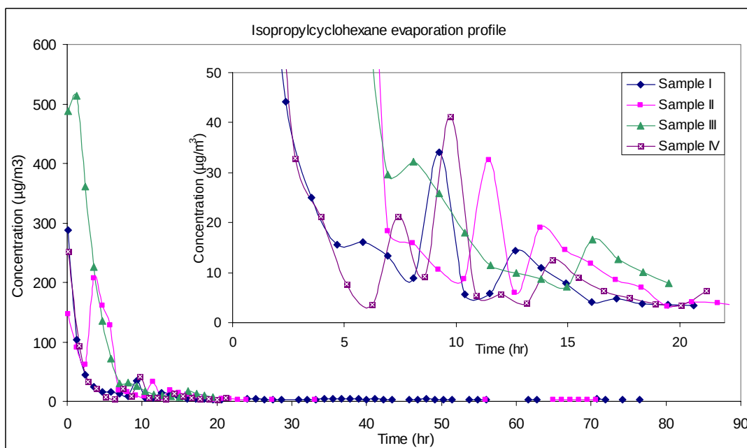
Figure 38. Concentration-time courses of isopropylcyclohexane in the vapor phase during evaporation of JP-8 samples I to IV at -10\text{ }^{\circ}\text{C} . The detection limit for this compound is \text{ca } 3\text{ }\mu\text{g}/\text{m}^3 .
