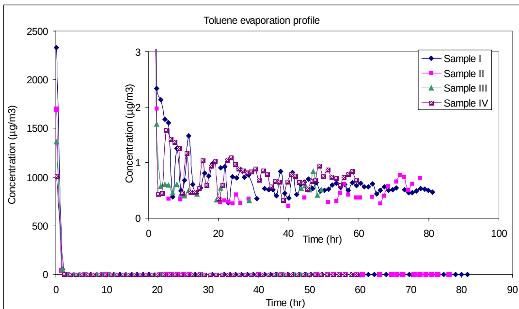
Figure 31. Concentration-time courses of toluene in the vapor phase during evaporation of JP-8 samples I to IV at -10^{\circ}\text{C} . The discontinuities in the measurements are due to the detection limit of the analytical configuration of \text{ca } 0.5 \mu\text{g}/\text{m}^3 .
