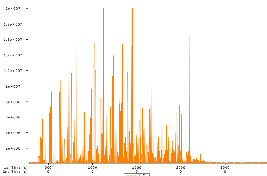
Figure 19. The modulated chromatogram (TIC) of the first vapor sample taken at 5 min after start of the evaporation of jet fuel sample I, the KC135 JP-8, at -10 °C.
