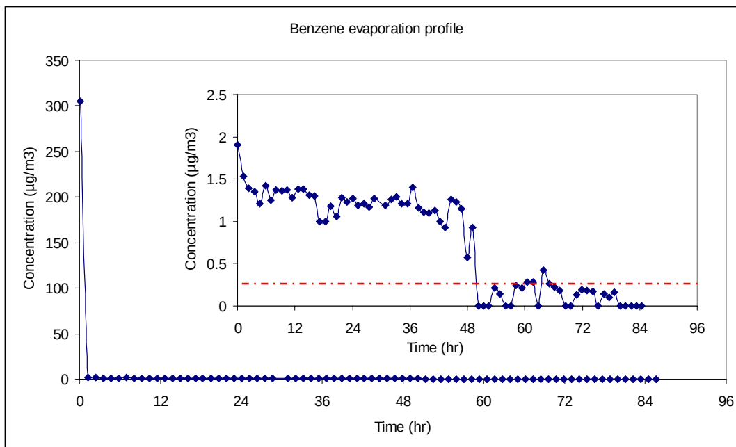
Figure 22. Concentration time course of benzene in the vapor phase during evaporation of JP-8 sample I (KC135) at -10 °C. The red line indicates the limit of detection of ca\ 0.2\ \mu\text{g}/\text{m}^3 for this particular component.
